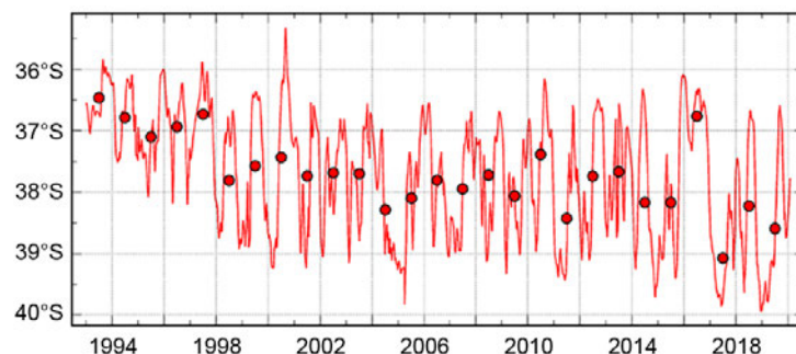
Fig. 3.19. Time series of the latitude of separation of the Brazil Current (BC) front from the continental shelf, defined as the intersection between the –1000-m bathymetry contour and the contour when the 10°C isotherm is 200 m deep. Solid red curve: 28-day running mean. Red dots: annual averages. The mean latitude of separation is 37.7°S ± 0.1°. (Source: www.aoml.noaa.gov/phod/altimetry/cvar/mal/BM_ts.php .)
