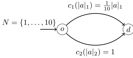
Fig. 1: Two link parallel congestion game. One edge possesses a linear congestion function, the other a constant congestion function. 10 users choose one of two resources: an upper path and lower path to traverse the network, i.e., \mathcal{A}_1 = \dots = \mathcal{A}_{10} = \{1, 2\} .
