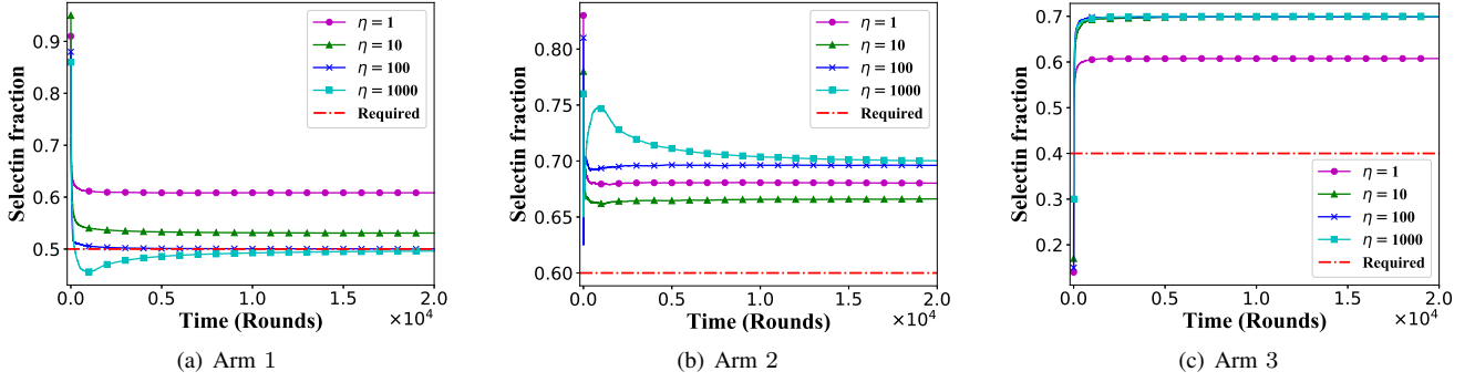
Fig. 5: Selection fraction over time under LFG with different values of \eta
