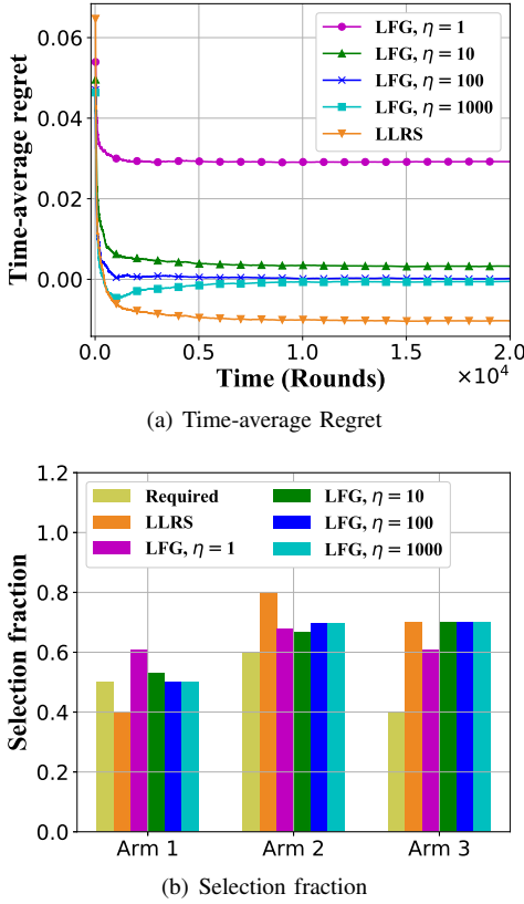
Fig. 4: Performance comparisons of different algorithms
