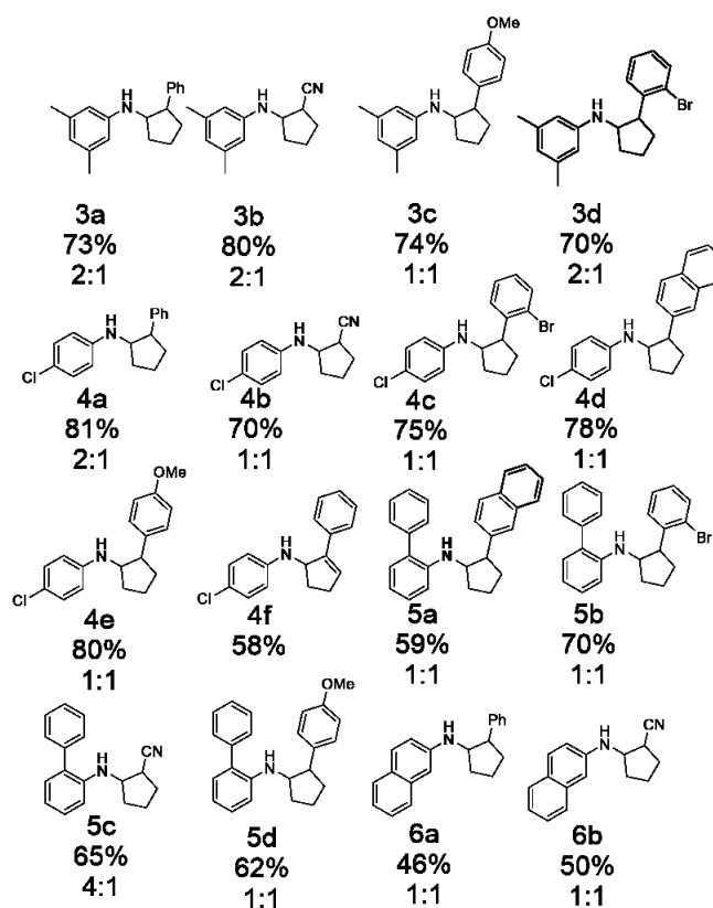
Scheme 3. The substrate scope of intermolecular [3+2] annulation by the electrochemical approach (percentages show the isolation yields)
