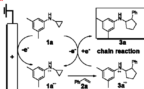
Scheme 1. Proposed mechanism for the [3+2] annulation reaction of N -cyclopropylanilines and styrene (top panel illustrates the reaction catalyzed with photocatalyst; bottom panel displays the reaction triggered electrochemically without using catalyst).
