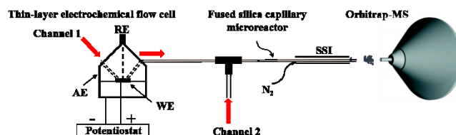
Scheme 2. Home-built electrochemistry/mass spectrometry (EC/MS) setup
