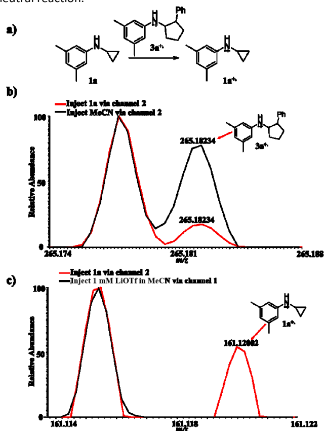
Figure 2. Online MS monitoring of the oxidation of 1a by 3a •+ : a) chemical equation showing the reaction between 1a and 3a •+ ; b) MS spectra showing the formation of the radical cation 3a •+ when the oxidation potential was applied to the cell. The signal of 3a •+ was lower when the solution injected via channel 2 changed from MeCN (black line) to 1a (red line). c) MS spectra showing the formation of radical cation 1a •+ (red line) when the cell was turned on with 3a being introduced into the flow cell via channel 1 and 1a being introduced via channel 2. No formation of radical cation 1a •+ was observed (black line) when the cell was turned on with 1 mM LiOTf in MeCN being introduced into the flow cell via channel 1 and 1a being introduced via channel 2.
