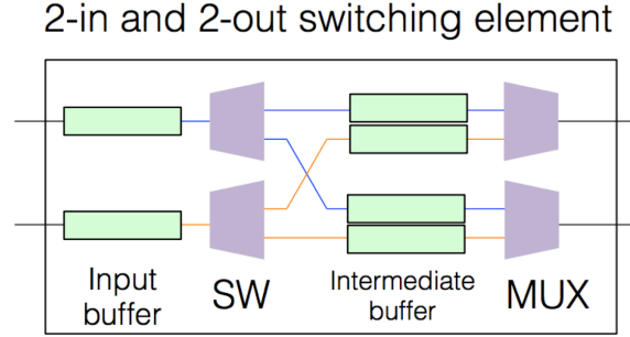
Figure 9: A single node in the Banyan switch showing input buffers and intermediate buffers. The buffers are 32 bits wide.
