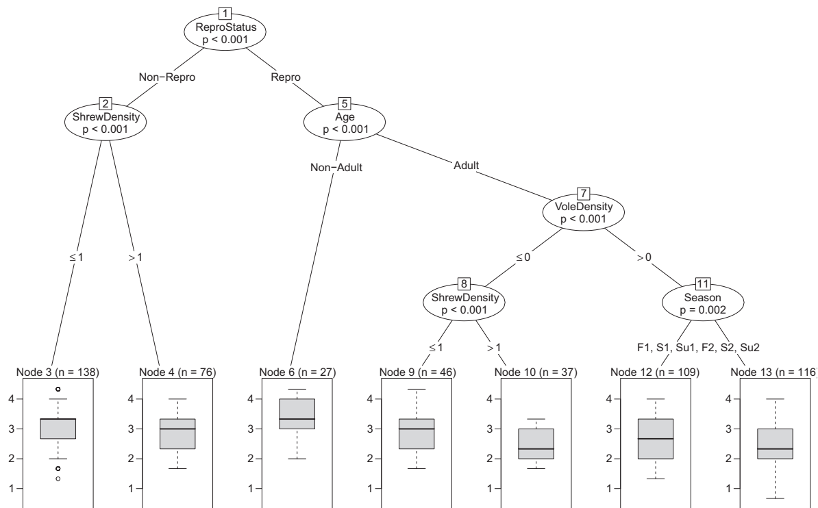
Fig. 4. Regression tree for body condition score of deer mice. Each terminal node provides a sample size with a box plot for that subgroup. “ReproStatus” stands for reproductive status. Juveniles and subadults were grouped together into “Non-Adult.” F1, S1, Su1, F2, S2, and Su2 represent fall/winter’16, spring’17, summer’17, fall/winter’17, spring’18, and summer’18, respectively. Density is per hectare. Statistical significance was set to 0.05.
