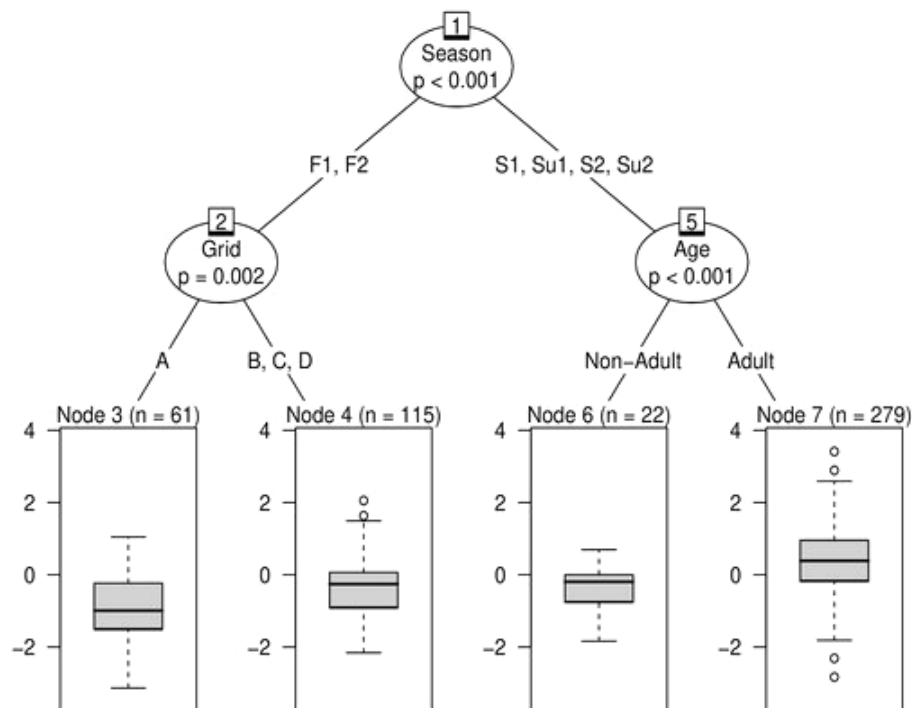
Fig. 3. Regression tree for ln neutrophil-to-lymphocyte (N/L) ratio of deer mice. Each terminal node provides a sample size with a box plot for that subgroup. Grids A and B were trapped from October'16 to July'18. Grids C and D were trapped from October'17 to August'18. Juveniles and subadults were grouped into "Non-Adult." F1, S1, Su1, F2, S2, and Su2 represent fall/winter'16, spring'17, summer'17, fall/winter'17, spring'18, and summer'18, respectively. Statistical significance was set to 0.05.
