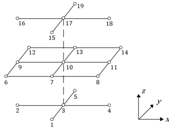
Figure 2. Lexicographical ordering of the 19-point stencil. Here, element 10 is the current point of the stencil [38].
