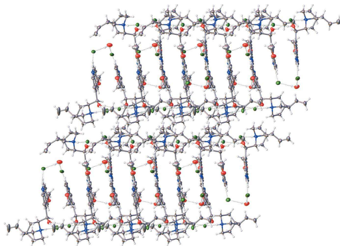
Figure 3 Packing diagram of the title compound viewed from the (110) plane.
