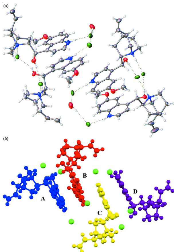
Figure 2 ( a ) The asymmetric unit of the title compound shown with 50% probability ellipsoids. Disorder is omitted for clarity. ( b ) The asymmetric unit colored to define the distinct cation pairs A and B (blue and red) and C and D (yellow and purple) discussed in the manuscript.
