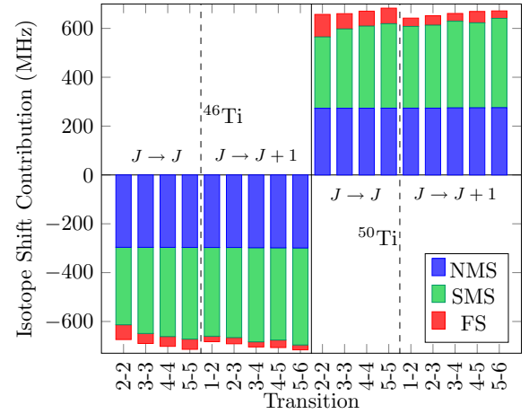
FIG. 4. The contributions to the overall isotope shifts due to the normal mass shift (NMS, blue), specific mass shift (SMS, green), and field shift (FS, red) for ^{46}\text{Ti} and ^{50}\text{Ti} , relative to ^{48}\text{Ti} . The contributions sum to the total isotope shift. The horizontal axis labels are the (J-J') pairs that define the transitions.
