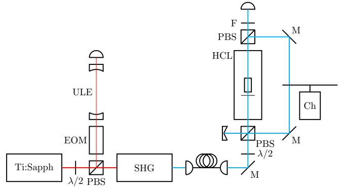
FIG. 2. The optical system. Infrared light is first generated with the Ti:sapph. Part of the light is sent through an electro-optic modulator (EOM) to an ultralow expansion cavity (ULE) for frequency referencing, and the rest of it is sent to the SHG stage. The frequency-doubled light is split into pump and probe beams, which counterpropagate through a hollow cathode lamp. A chopper (Ch) amplitude modulates the pump beam. A filtered photodiode detects the probe beam. Key: M, mirror; \lambda/2 , half-wave plate; PBS, polarizing beam splitter; and F, filter.
