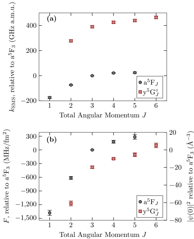
FIG. 6. The (a) specific mass shift and (b) field shift coefficients for the 10 levels investigated, reported relative to a^5F_3 . The value of F is proportional to the electron density at the nucleus [(b), right axis].
