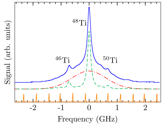
FIG. 3. Saturated absorption spectrum of the a^5F_5 \rightarrow y^5G_6^o transition in titanium. The signal (blue, upper) obtained following demodulation at the chopping frequency shows clear peaks for the three I = 0 isotopes: ^{46}\text{Ti} , ^{48}\text{Ti} , and ^{50}\text{Ti} . The peak frequencies are obtained by fitting the observed spectrum as 10 Lorentzians (green, dashed) on top of the Gaussian background (red, dot-dashed) that is produced by diffusion of the excited-state atoms (see text). The number of Lorentzian peaks used in the fitting was chosen to capture as much of the fermionic resonances as detectable without over-constraining the model. ULE transmission resonances (orange, bottom), obtained simultaneously using the electro-optically modulated fundamental laser light, generate calibration frequency markers for the frequency-doubled light used in spectroscopy.
