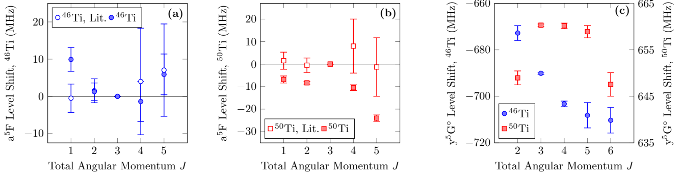
FIG. 5. Isotopic level shifts of the a^5F manifold [panels (a) and (b)] and the y^5G^o manifold [panel (c)] for ^{46}\text{Ti} (blue circles) and ^{50}\text{Ti} (red squares), relative to the a^5F_3 level. Literature values [14] (open symbols) are plotted where known.
