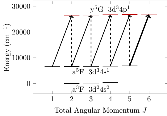
FIG. 1. The relevant energy levels in titanium. The a^5F_5 metastable state supports a near-cycling transition (bolded) to the y^5G_6^o state. The J \rightarrow J+1 transitions (solid) and J \rightarrow J transitions (dashed) together can be used to determine the level shifts of all of the levels in the a^5F_J and y^5G_J^o manifolds. Black levels are even parity, and red (upper) levels are odd parity.
