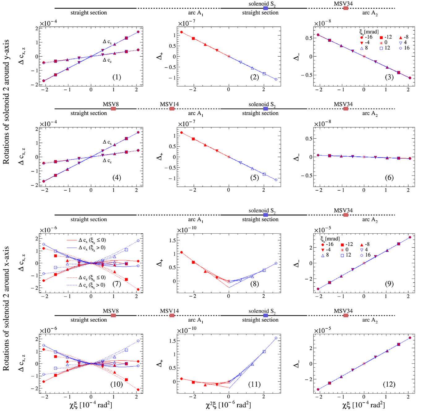
FIG. 10. Perturbation of the spin transfer matrix \mathbf{t}_R [see Eq. (58)] due to closed orbit excursions (see Fig. 8) by the steering fields of the misaligned solenoid S_2 . Panels 1–6 show the effect of rotations of solenoid S_2 around the y-axis. The first row of panels 1–3 shows \Delta c_{x,z}(\xi, \chi_{AI}) [Eq. (64)], and \Delta_{\pm}(\xi, \chi_{AI}) [Eq. (65)] for orbit set 1 (Table III). The second row of panels 4–6 show the same parameters for orbit set 2. The corresponding situation for rotations of S_2 around the x-axis is depicted in panels 7–12. Note that in order to emphasize the different scaling properties, \Delta c_{x,z} (first column of panels) and \Delta_- (third column) are plotted as a function of the variable \chi \xi , while \Delta_+ (second column) is plotted as a function of the variable \chi^2 \xi . To avoid overcrowding of data points, for each \xi only the end point results at \chi_{AI} = \pm 12.98 mrad are shown. In panels 1 to 6, 9 and 12, the points for all \xi fall on the same straight line. In panels 7, 8, 10, and 11, the actual dependence on \chi_{AI} is shown by the curves drawn to guide the eye (see text for more explanations).
