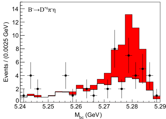
FIG. 5. Distribution of the M_{\text{bc}}^{\text{sig}} for the B^- \rightarrow D^{*0} \pi^- \eta sample. The solid histogram shows the MC distribution (the red-filled and the white components for the correct B and fake B candidates, respectively) and the black dots are the data distribution.
