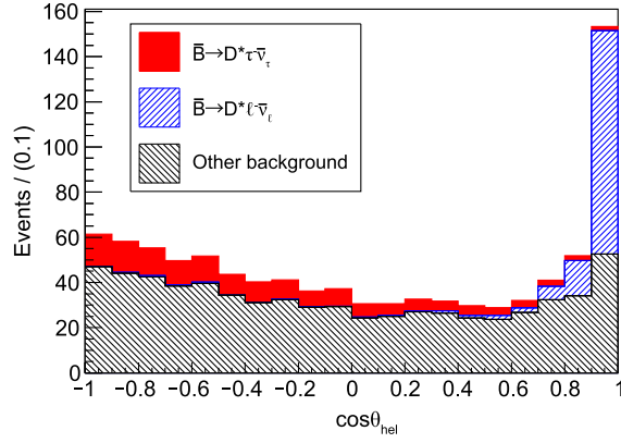
FIG. 2. Distribution of \cos \theta_{\text{hel}} (MC) for the signal (red), \bar{B} \rightarrow D^* \ell^- \bar{\nu}_\ell (blue-hatched) and the other background (black-hatched) in the \tau^- \rightarrow \pi^- \nu_\tau sample. The SM prediction on P_\tau(D^*) is assumed. All the signal selection requirements including E_{\text{ECL}} and q^2 are applied.
