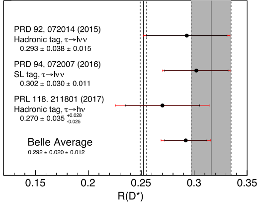
FIG. 11. Summary of the R(D^*) measurements based on the full data sample of Belle and their average. The inner (outer) error bars show the statistical (total) uncertainty. The shaded band is the world average as of early 2016 [20] while the white band is the SM prediction [23]. On each measurement, the tagging method and the choice of the \tau decay are indicated, where “SL tag” is the semileptonic tag and h in the \tau decay denotes a hadron h = \pi or \rho .
