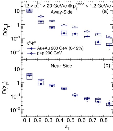
Fig. 2. (Color online.) The z_T dependence of \pi^0 - h^\pm away-side (a) and near-side (b) associated charged-hadron yields per trigger for Au+Au at 0–12% centrality (filled symbols) and p + p (open symbols) collisions at \sqrt{s_{NN}} = 200 GeV. Vertical lines represent the statistical errors, and the vertical extent of the boxes represents systematic uncertainties.
