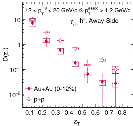
Fig. 3. (Color online.) The z_T dependence of \gamma_{dir} - h^\pm away-side associated charged-hadron yields per trigger for Au+Au at 0–12% centrality (filled diamonds) and p + p (open diamonds) collisions. Vertical lines represent statistical errors, and the vertical extent of the boxes represents systematic uncertainties.
