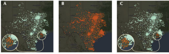
Fig. 4. Evaluation of the boundary defense mechanism. (A) The grid is under “zonal attack,” where the measurements within a zone are corrupted (shown in red). SE based on (B) Newton’s method for nonlinear least squares, and (C) the proposed method with SOC, where in both cases, buses with an estimation error greater than 0.002 are marked in red.
