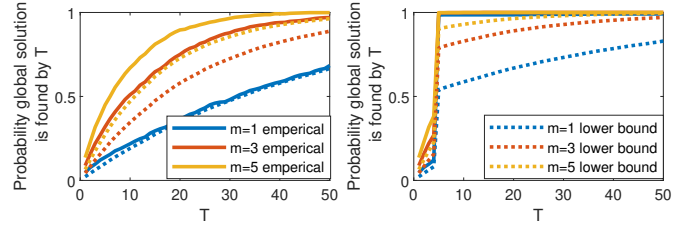
Fig. 3. Empirical validation of Theorem 1.
