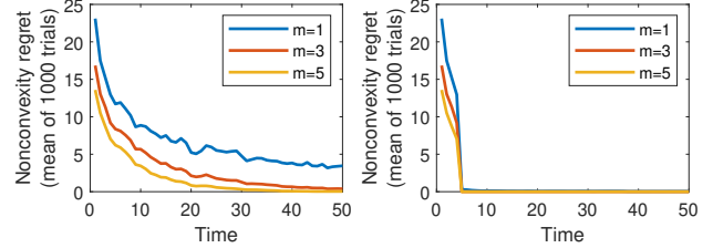
Fig. 4. Nonconvexity regret over time resulting from applying Algorithm 1 to Case 1 (left) and Case 2 (right).
