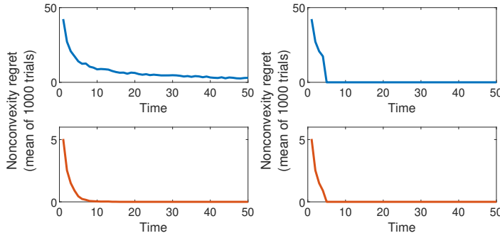
Fig. 5. Nonconvexity regret over time resulting from applying Algorithm 2 to Case 1-b (left) and Case 2-b (right), with parameters \alpha = 0.1, \delta = 0.1, \bar{m} = 5 (top) and \alpha = 0.1, \delta = 0.9, \bar{m} = 125 (bottom).
