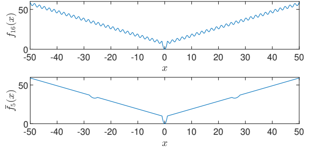
Fig. 1. Top and bottom plots show examples of a problem with high and low complexity, respectively.
