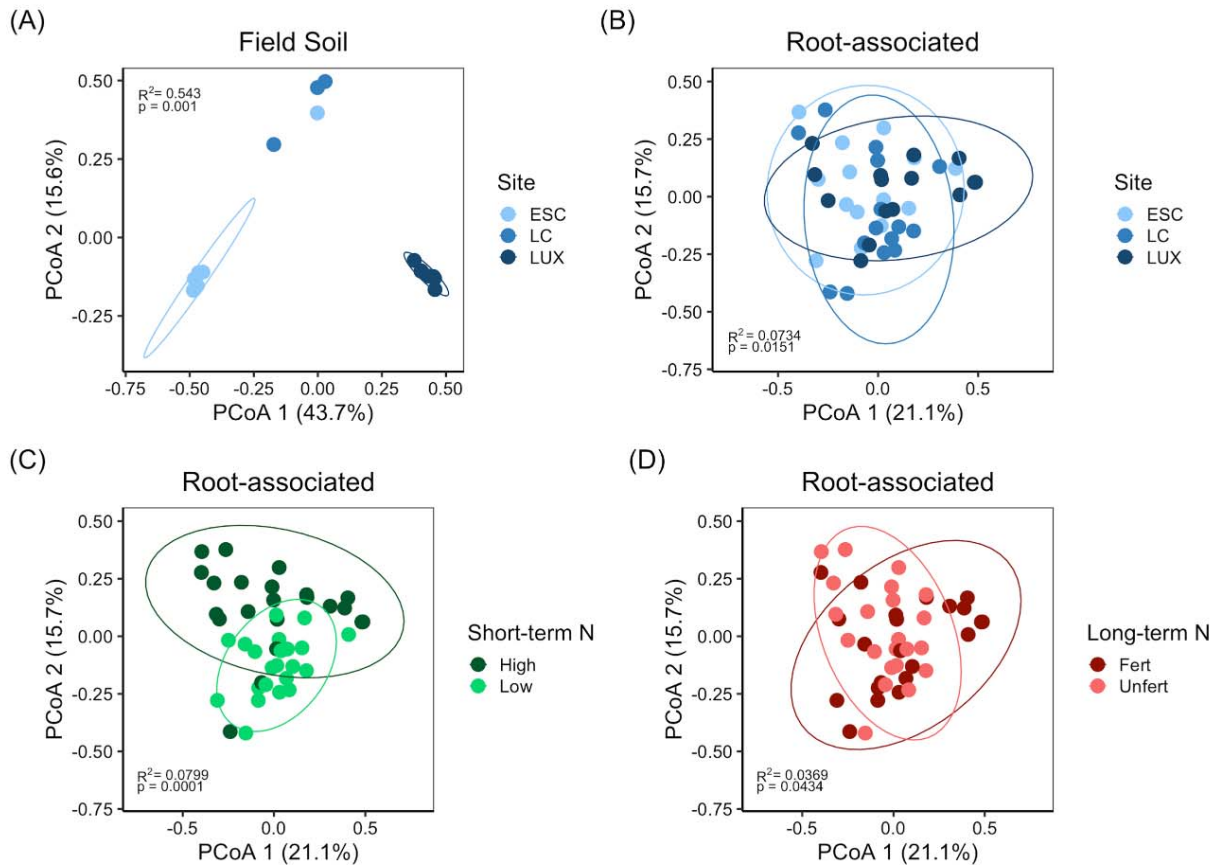
Figure 3: Principal coordinates analysis of (A) field soil and (B) root-associated samples colored by site, (C) by short-term N treatment, and by (D) long-term N treatment. Points are based on Bray-Curtis distance matrix of the relative abundance of rarefied OTU counts. Each point represents one replicate. Ellipses represent 95% confidence ellipse of the centroid. Note that LC field soil does not have an ellipse because only 3 soil samples (of the 8 total) amplified for nifH and were sequenced.
