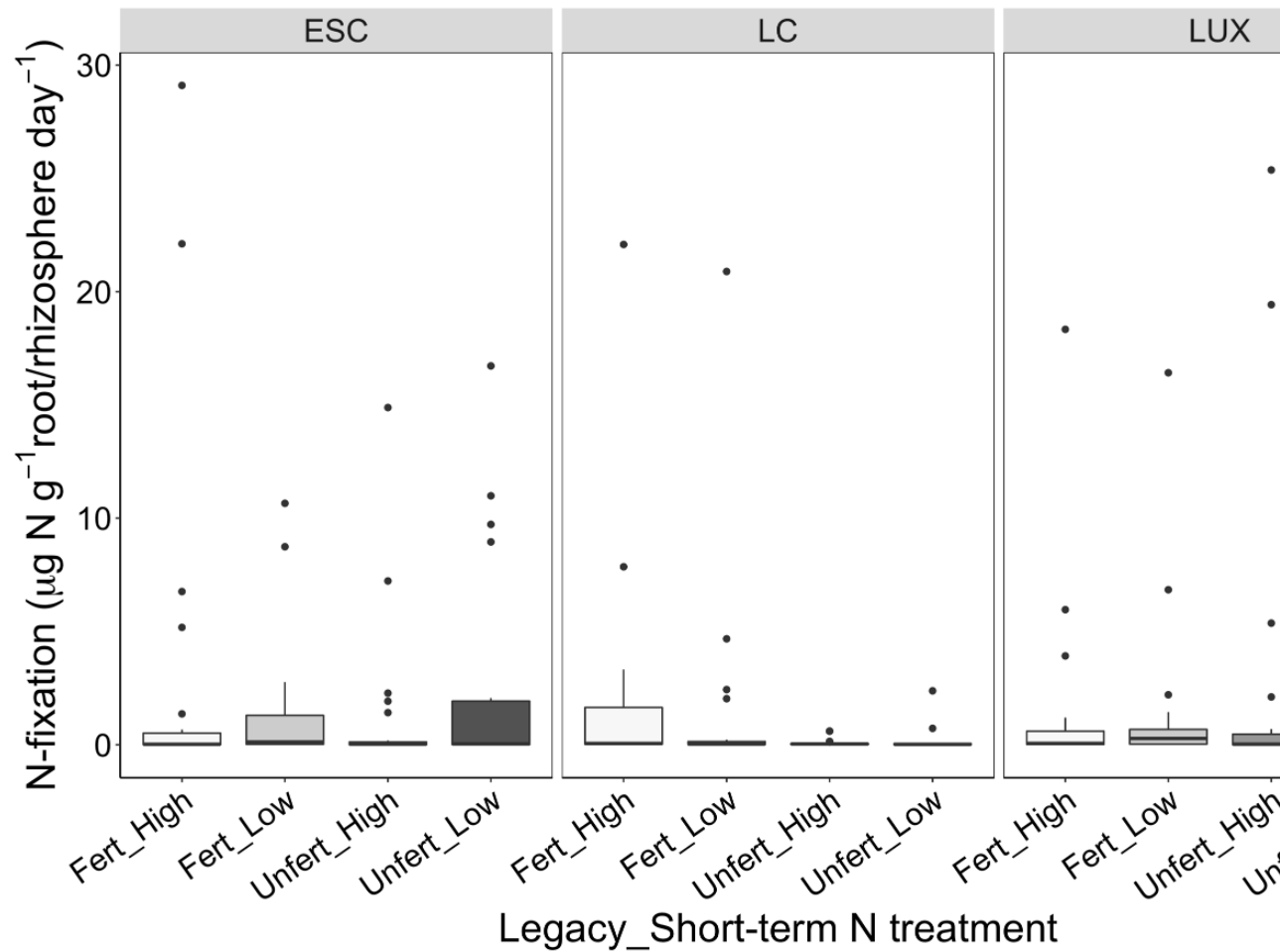
Supp. Fig. 3: Root-associated nitrogen fixation rates for each site (ESC = Escanaba, LC = Lake City, LUX = Luleå), by the long-term and short-term N treatments (F_High = Fertilized field + High N addition in greenhouse, F_Low = Fertilized field + Low N greenhouse, U_High = Unfertilized field + High N greenhouse, U_Low = Unfertilized field + Low N greenhouse). Boxplots show full range of N-fixation values for all pseudoreplicates in each treatment with horizontal bars representing average N-fixation (n = 24 per bar).
