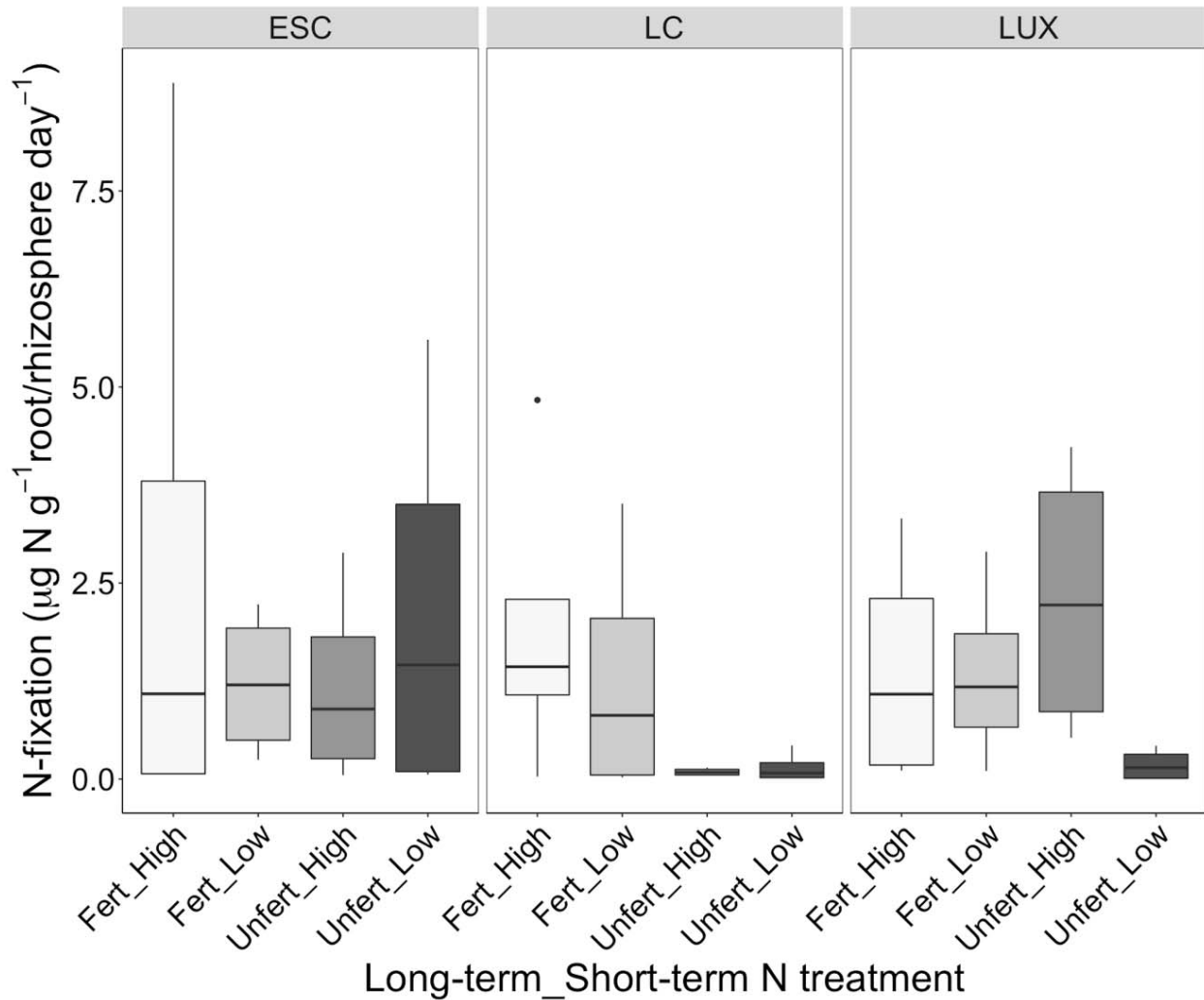
Figure 6: Root-associated nitrogen fixation rates for each site (ESC = Escanaba, LC = Lake City, LUX = Lux Arbor) by the long-term and short-term N treatments (F_High = Fertilized field + High N addition in greenhouse, F_Low = Fertilized field + Low N greenhouse, U_High = Unfertilized field + High N greenhouse, U_Low = Unfertilized field + Low N addition). Boxplots show full range of N-fixation values for each treatment with solid black horizontal bars representing average N-fixation (n = 4 per bar).
