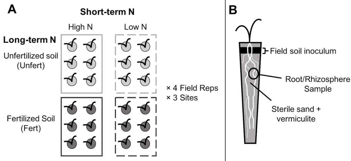
Figure 1: Experimental design of (A) N treatments and (B) planting. There were 6 analytical replicate pots per long-term x short-term N treatment combination. This was repeated for each field block (4 per site) and each field site (3 – Escanaba, Lake City, and Lux Arbor) for a total of 288 analytical replicate pots and 48 experimental units. Field soils were used to inoculate pots by adding a thin layer of soil near the surface of each pot
