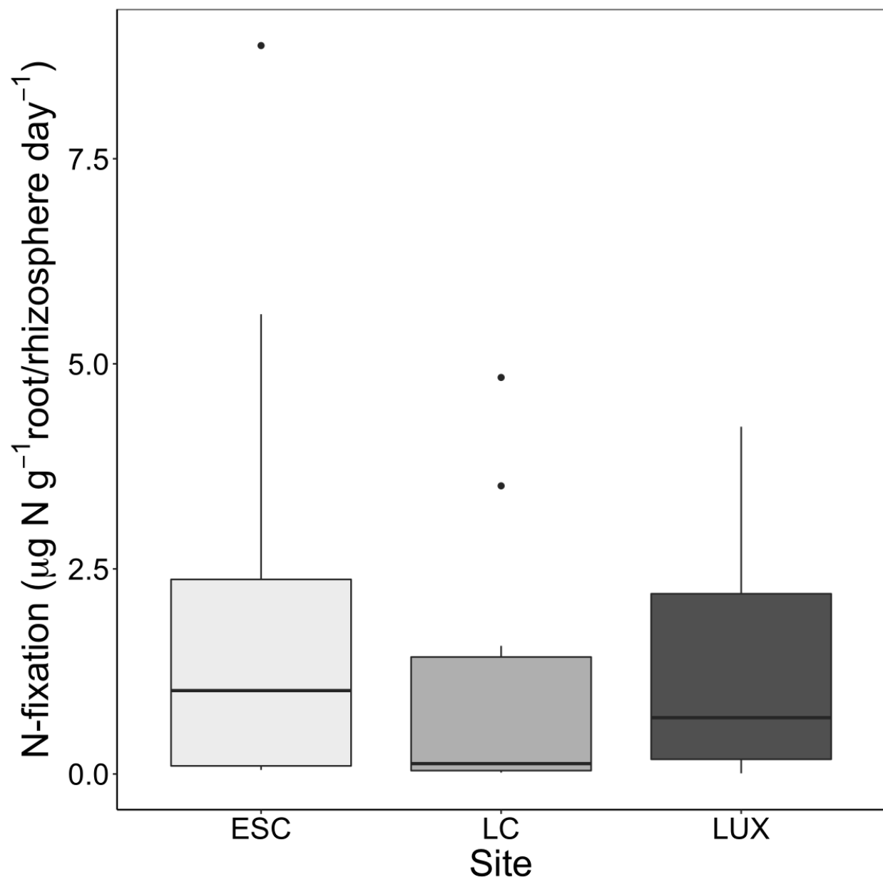
Supp. Fig. 2 nitrogen fixation at each site, average N-fixation for each treatment and short-term N-fixation. Box plots show full range of values for each treatment with horizontal bars showing average N-fixation (horizontal bar).
