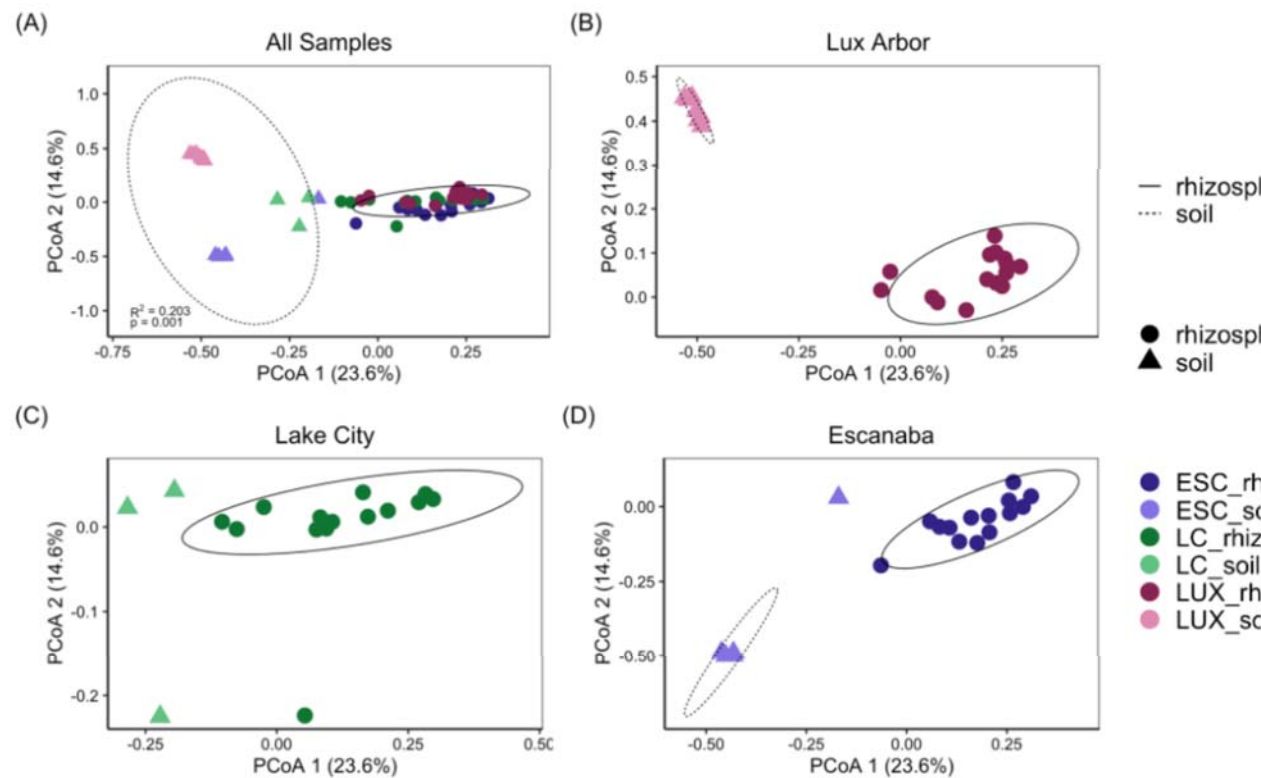
Supp. Fig. 5: Principal coordinates analysis of field soil samples (soils used to inoculate the greenhouse associated samples (from switchgrass plants grown in greenhouse soil) for (A) All samples, (B) Lux Arbor, (C) Lake City, and (D) Escanaba. Points are based on a Bray-Curtis distance matrix of the relative abundance of rare taxa. Points are colored by site by sample type with shape representing sample type (e.g. field soil or rhizosphere). Ellipses represent 95% confidence ellipse of the centroid for each sample type. Samples do not have an ellipse because only 3 soil samples (of the 8 total) amplified for nifH and were included in the analysis.
