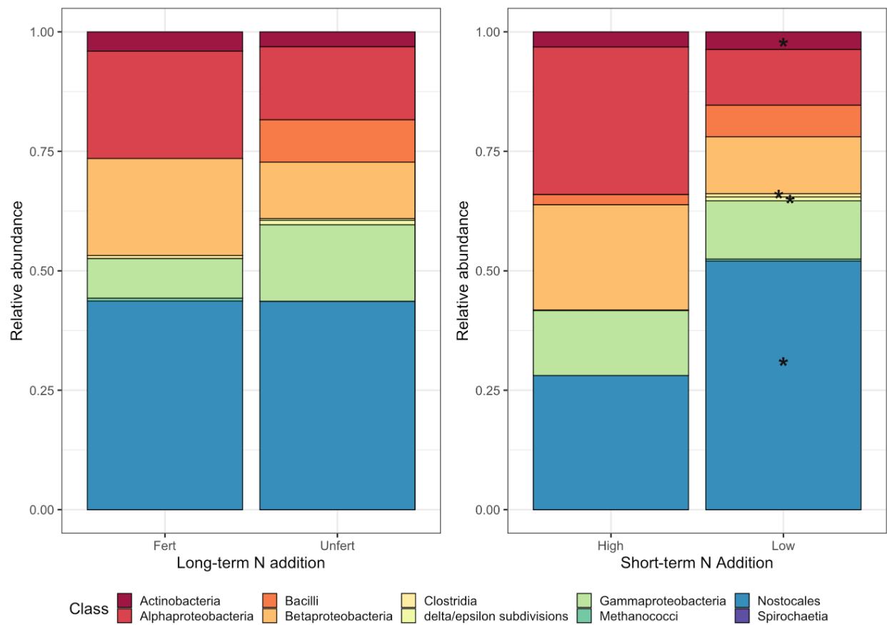
Figure 5: Average relative abundance of diazotroph classes by long-term N (Fert = Fertilized, Unfert = Unfertilized) and short-term N additions (High = High N addition, Low = Low N addition) for root-associated samples. Asterisks indicate significant difference in diazotroph class by N treatment at p < 0.05 with asterisk placed on the bar with greater relative abundance. Each bar represents the average of 24 samples.
