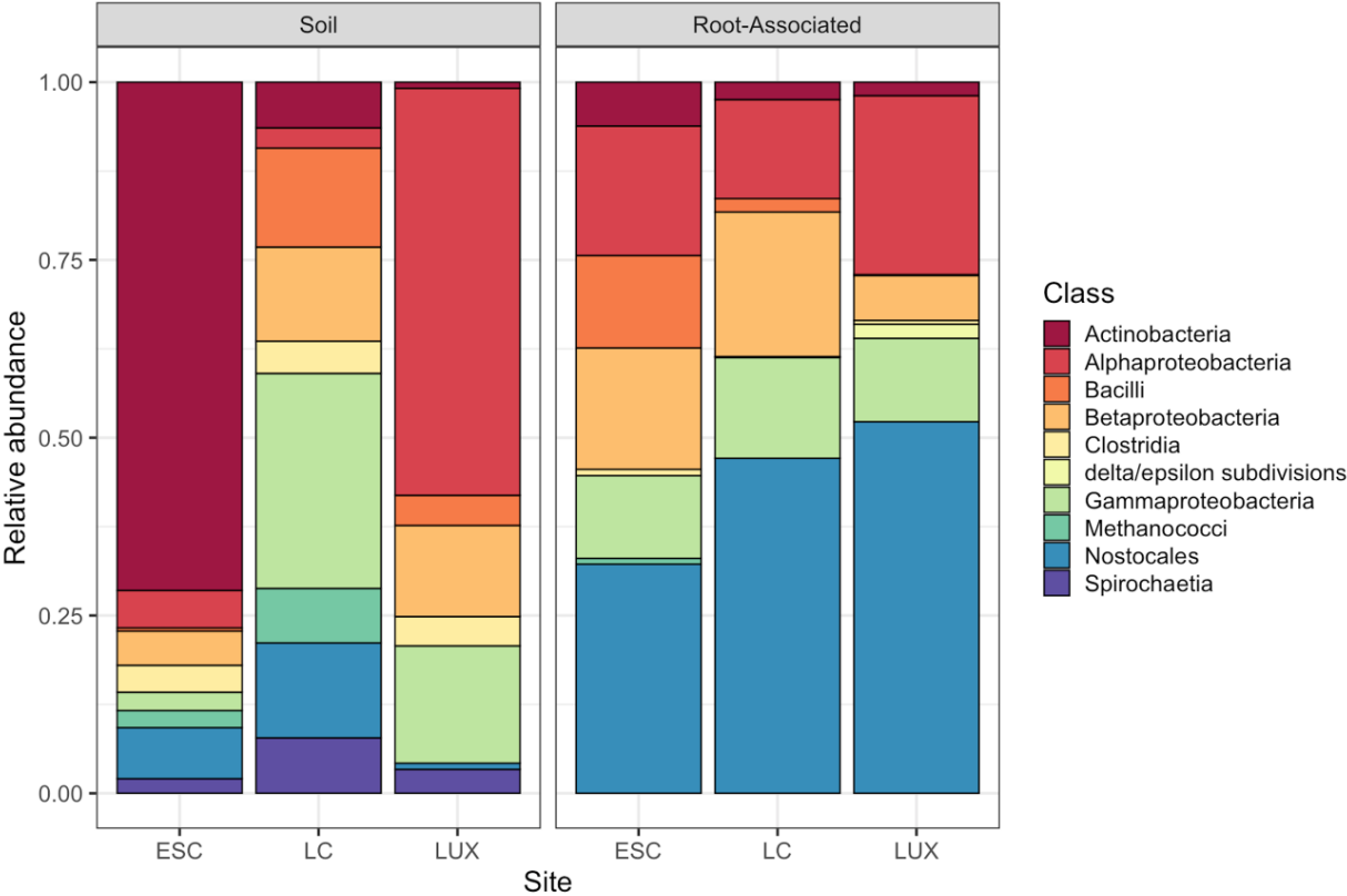
811 Figure 4: Average relative abundance of diazotroph classes by site (ESC = Escanaba, LC = Lake 812 City, LUX = Lux Arbor) for soil (those soils used to inoculate the greenhouse pots) and root- 813 associated samples. Bars represent the average of 8 samples for soil (only 3 for LC) and 16 814 samples for roots. Full results are presented in Table 2.
