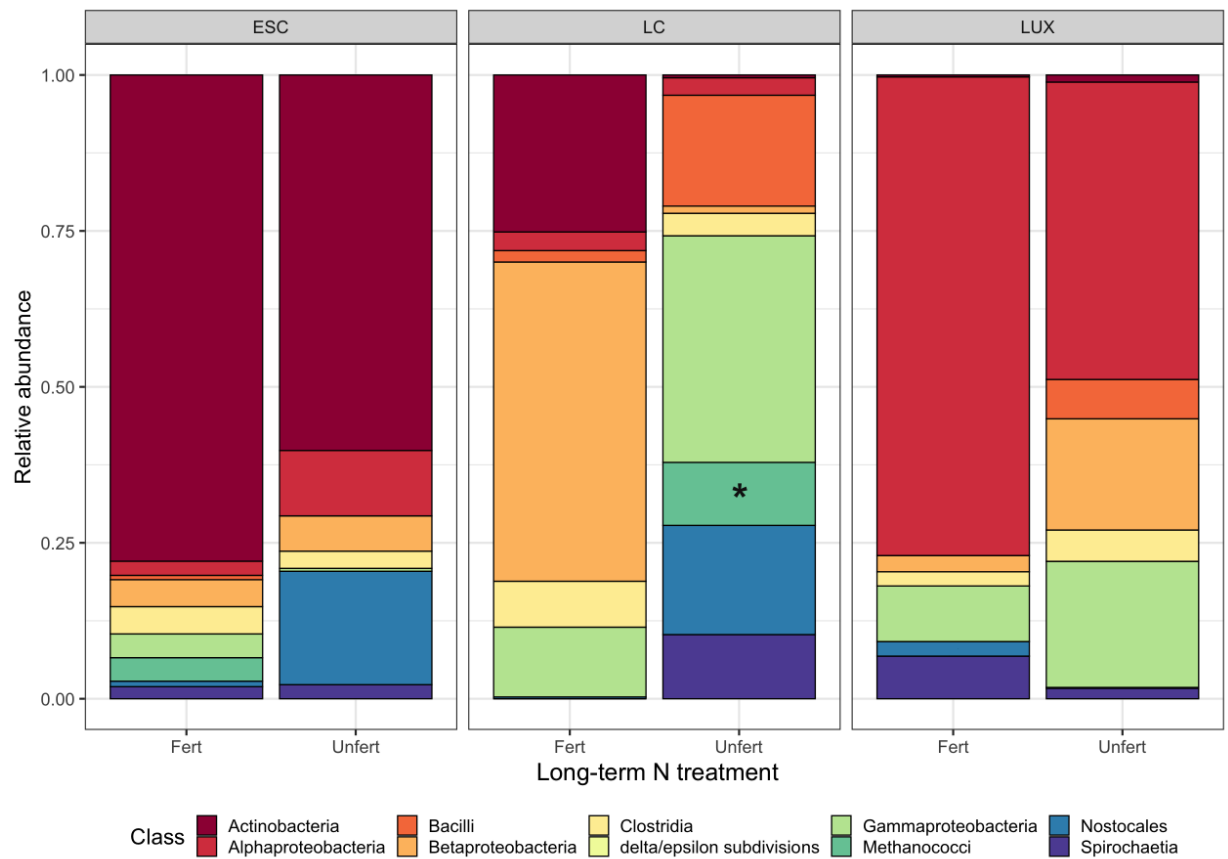
Supp. Fig. 1: Average relative abundance of diazotroph classes by long-term N treatment and site for . Asterisks indicate a significant difference between long-term N treatments within sites at p < 0.05 and of greater relative abundance. Only the relative abundance of Methanococci at LC was found to differ between long-term N treatments. Bars for ESC and LUX represent the average of 4 samples. LC bars 1 sample for Fert and 2 samples for Unfert.
