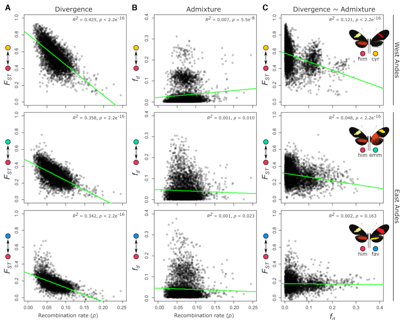
Figure 6. Correlations of divergence and admixture proportions with recombination rate in the three H. himera – H. erato contact zones. (A) Relative divergence ( F_{ST} ) versus population recombination rate ( \rho ). (B) Admixture proportion ( f_d ) versus population recombination rate ( \rho ). (C) Relative divergence ( F_{ST} ) versus admixture proportion ( f_d ). Statistics were calculated in 50 kb non-overlapping windows. Recombination rates were calculated from each H. erato population separately and averaged over populations (see methods) and showed a genome-wide average of \rho equal to 0.071 (SD = 0.026; \rho = 4N_e r ). Colored circles match geographic distributions and contact zones in Figure 2.
