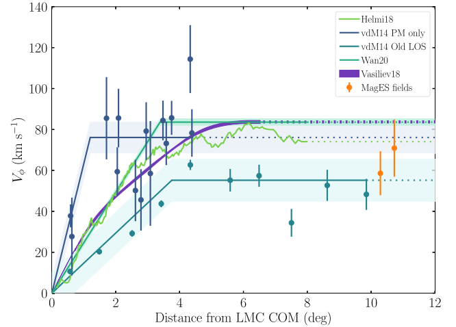
Figure 9. Azimuthal velocities in the LMC disc as a function of distance from the LMC COM. Orange points indicate measurements for the two MagES fields in the northern LMC disc; error bars include propagated uncertainties from all parameters. Dark blue points show van der Marel & Kallivayalil (2014) values derived from HST proper motion measurements of mixed young and old populations, while light blue/aqua points show van der Marel & Kallivayalil (2014) values derived from LOS observations for their ‘old’ stellar population. Error bars on these points only include uncertainty in the observed motions, and not disc geometry or COM location, and are thus smaller than those for the MagES fields. The solid lines reflect the best-fitting rotation models derived from Vasiliev (2018) (labelled Vasiliev18), Wan et al. (2020) (labelled Wan20), Gaia Collaboration (2018c) (labelled Helmi18), and van der Marel & Kallivayalil (2014) (labelled vdM14). Surrounding shaded regions indicate 1\sigma uncertainty propagated from all parameters; these are thus comparable to the error bars of the MagES fields. Dashed continuations of the solid lines indicate where these models have been extrapolated outwards in order to facilitate comparison with the two MagES points. The observations used to derive the velocities shown are generally located much closer to the LMC COM than the MagES fields.
