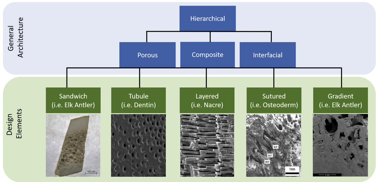
Fig. 5 – General architecture and specific design elements found in biological materials and, more particularly, impact resistant materials. (Top) Four general features found in all biological materials that are especially important for impact resistance. All biological materials are hierarchical. These hierarchies are composed of various arrangements of composite materials, pores, and interfaces. (Bottom) Five micro- and meso-structures that are commonly found in impact resistant biological materials and have been shown to improve performance under dynamic loading. These include sandwich, tubule, layered, sutured [62], and gradient structures. Adapted with permission [62] Copyright 2015, Acta Materialia.
