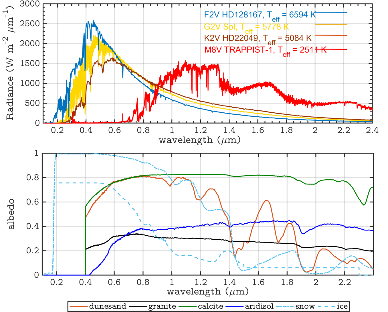
Figure 1. Top: Spectral energy distribution (SED) of TRAPPIST-1 (red) (Lincowski et al., 2018), compared to those of standard main sequence F- and K- dwarf stars (Segura et al., 2003) (not used in this work and presented here for comparison only). The solar spectrum, which was used to initialize some control runs, is from Chance & Kurucz (2010). See Rushby et al. (2019) or Shields et al. (2013) for details regarding the reduction of these spectra. Bottom: the spectral distribution of the surface compositions used in this work: dunesand (brown/red), granite (black), calcite (green), aridisol (blue), as well as fine-grained snow (dash-dotted light blue) and blue marine ice (dashed light blue).
