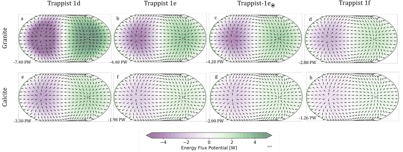
Figure 7. Energy Flux Potential ( \chi ) (W) for planets TRAPPIST-1d, e, e modelled with a solar spectrum, and TRAPPIST-1f using granite (top row) and calcite (bottom row) land surface compositions. Vectors are normalized divergent energy flux potential. Negative (purple) energy flux potential values occur on the day side of the planet, while positive (green) energy flux potential values occur on the night side of the planet. The minimum \chi for each simulation is noted in the lower left of each panel (and in table 2)
