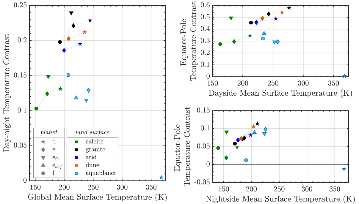
Figure 5. Left: Dayside-to-nightside temperature contrast ( [T_{day} - T_{night}]/T_{equil} ) (K) and global mean surface temperature (K). Icons denote planet d , e , f , planet e modelled using a solar spectrum ( e_{\odot} ), and planet e modelled using CESM’s default snow and ice albedos ( e_{def} ) (only for aquaplanet simulations). Colors represent land surface type; calcite: green, granite: black, aridisol: dark blue, dunesand: brown/red, aquaplanet: light blue. Top right: Dayside equator-to-pole temperature contrast ( [T_{equator} - T_{polar}]/T_{equil} ) as a function of dayside mean surface temperature. Bottom right: Nightside equator-to-pole temperature contrast ( [T_{equator} - T_{polar}]/T_{equil} ) as a function of nightside mean surface temperature. Note the differing ranges of the y-axis between the figures on the right: the equator-to-pole temperature contrast is larger on the dayside than the nightside.
