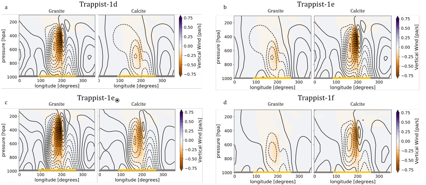
Figure 9. Global east-west overturning circulation at the equator ( \text{kg/s} ) (Walker circulation) for homogeneous surface composition TRAPPIST-1 planets – granite (left), calcite (right). Yellow shading denotes the dayside and gray the nightside (i.e., substellar centered at 180^\circ ). Contour intervals are 1 \times 10^{10} \text{ kg/s} , with solid contours indicating clockwise and dashed contours indicating counter-clockwise circulation. Shading denotes vertical wind speed ( \text{pa/s} ), where positive values denote vertically upwards flow.
