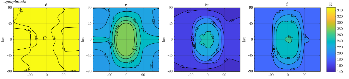
Figure 4. Contours (interval 20 K, except d where intervals are 2 K) of surface temperature as a function of latitude and longitude for aquaplanet d , e , e_{\odot} , and f .
