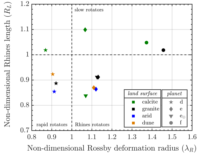
Figure 6. Rotational regimes for TRAPPIST-1 planets and land surfaces considered in this work. Tidally-locked planets are in the rapidly rotating regime when the non-dimensional Rossby deformation radius is less than one, which includes most land composition scenarios for TRAPPIST-1d (pentagram markers); TRAPPIST-1f (circle markers) falls into a slow rotator regime, and most simulations for TRAPPIST-1e suggest that the planet is a Rhines rotator, except in the case of the calcite simulation.
