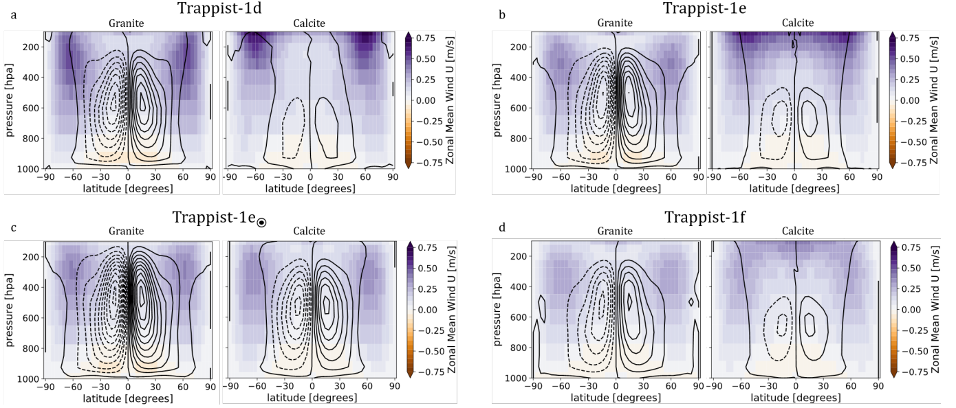
Figure 8. Mean meridional overturning circulation ( \text{kg s}^{-1} ) (Hadley cell) for homogeneous surface composition TRAPPIST-1 planets – granite (left), calcite (right). Contour intervals are 2.5 \times 10^{10} \text{ kg s}^{-1} , with solid contours indicating clockwise and dashed contours indicating counter-clockwise circulation. Shading denotes zonal mean wind speed ( \text{m s}^{-1} ).
