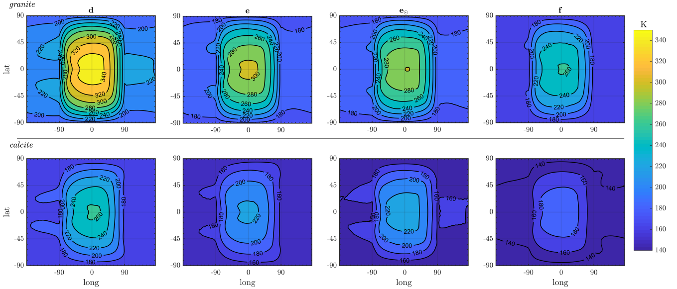
Figure 3. Top row: Contours (interval 20 K) of average surface temperature as a function of latitude and longitude for planet d , e , e modelled using a solar spectrum ( e_\odot ), and f for a homogeneous granite surface. Bottom row: Contours (interval 20 K) of surface temperature as a function of latitude and longitude for planet d , e , e_\odot , and f for a homogeneous calcite surface.
