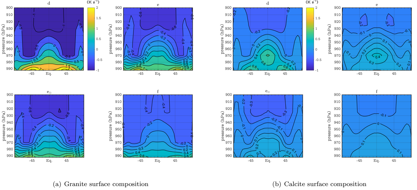
Figure 11. Globally-averaged contours of atmospheric heating ( Q_R ) ( \text{K s}^{-1} ) as a function of latitude and pressure (lower atmosphere ( >900 hPa) plotted) for granite surfaces (left two columns (a)) and calcite surfaces (right two columns (b)) on TRAPPIST-1d (top left), e (top right), e_o (bottom left), and f (bottom right).
