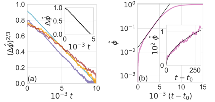
FIG. 5. Topological characteristics of the time dependence of phase amplification for \ell = 100 . (a) For spherical domains, the reduced deviation from the equilibrium order parameter, \Delta\hat{\phi} = 1 - \phi/\phi_0 scales as t^{3/2} . This is shown for temperatures, \Delta\hat{T} , as 0.11 (cyan), 0.025 (purple), 0.014 (orange), and 0.009 (brown). The inset shows the effect for a cylindrical domain at \Delta\hat{T} = 0.11 . (b) A zero curvature Schwarz-P interface is initially formed by simulating a system with Kawasaki dynamics ( p_r = 0 ) for a long time. At t - t_0 = 0 , the system obtains Glauber dynamics ( p_r = 1 ), and the collapse of one of the phases is shown. One can see a transitions from random-walk behavior, \sqrt{t} , at short times (see inset) to exponential behavior (straight line) before saturation.
