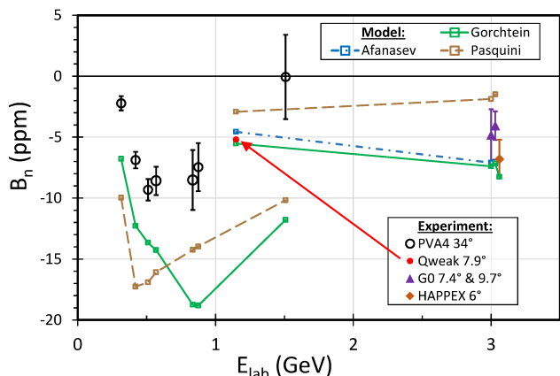
FIG. 3. Beam energy dependence of all forward-angle ( \theta_{\text{lab}} \leq 34^\circ ) elastic ep B_n data compared to calculations at each experiment's kinematics. The far-forward angle (solid symbols, \theta_{\text{lab}} < 10^\circ ) are from this experiment (red circle, uncertainty smaller than the symbol), G0 [24] (purple triangles), and HAPPEX [25] (orange diamond). Less forward-angle data \theta_{\text{lab}} \approx 34^\circ are denoted with open circles from PVA4 [26, 27] (black). The predictions (open squares) from each theoretical group (Pasquini & Vanderhaeghen [4, 5], Afanasev & Merenkov [10, 11], and Gorchtein [3, 6–9]) are connected by straight-line segments for the far-forward and the forward angle calculations, to help guide the eye.
