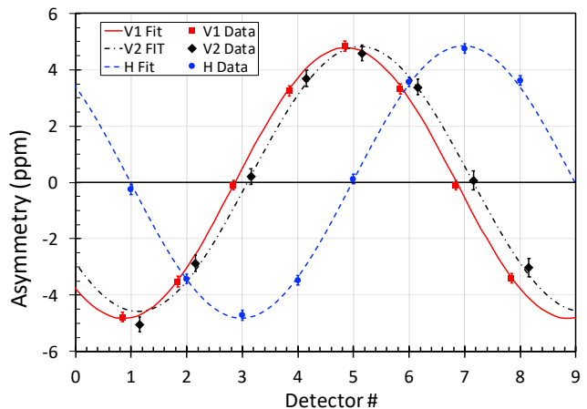
FIG. 1. Extraction of the experimental asymmetry A_{\text{exp}} from the measured asymmetries A_{\text{msr}}^i for the horizontal (H) and the two vertical data sets (V1 and V2). The phases of the vertical data sets were offset -7^\circ (V1) and +7^\circ (V2) in the figure for clarity. The detector number corresponds to the azimuthal location of the detectors, starting from beam left (Detector 1) where \phi_i = 0^\circ , and increasing clockwise every 45^\circ . Uncertainties shown are statistical only. The reduced \chi^2 (5 degrees of freedom) in the fits are 0.15 (V1), 1.07 (V2), and 0.81 (H).
