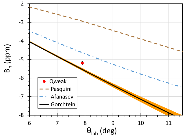
FIG. 2. Comparison of this measurement (red circle) to calculations at E_{\text{lab}} = 1.149 \text{ GeV} by Pasquini & Vanderhaeghen [4], Afanasev & Merenkov [10], and Gorchtein [6] over the Q_{\text{weak}} acceptance. The orange band about the latter calculation indicates the model uncertainty.
