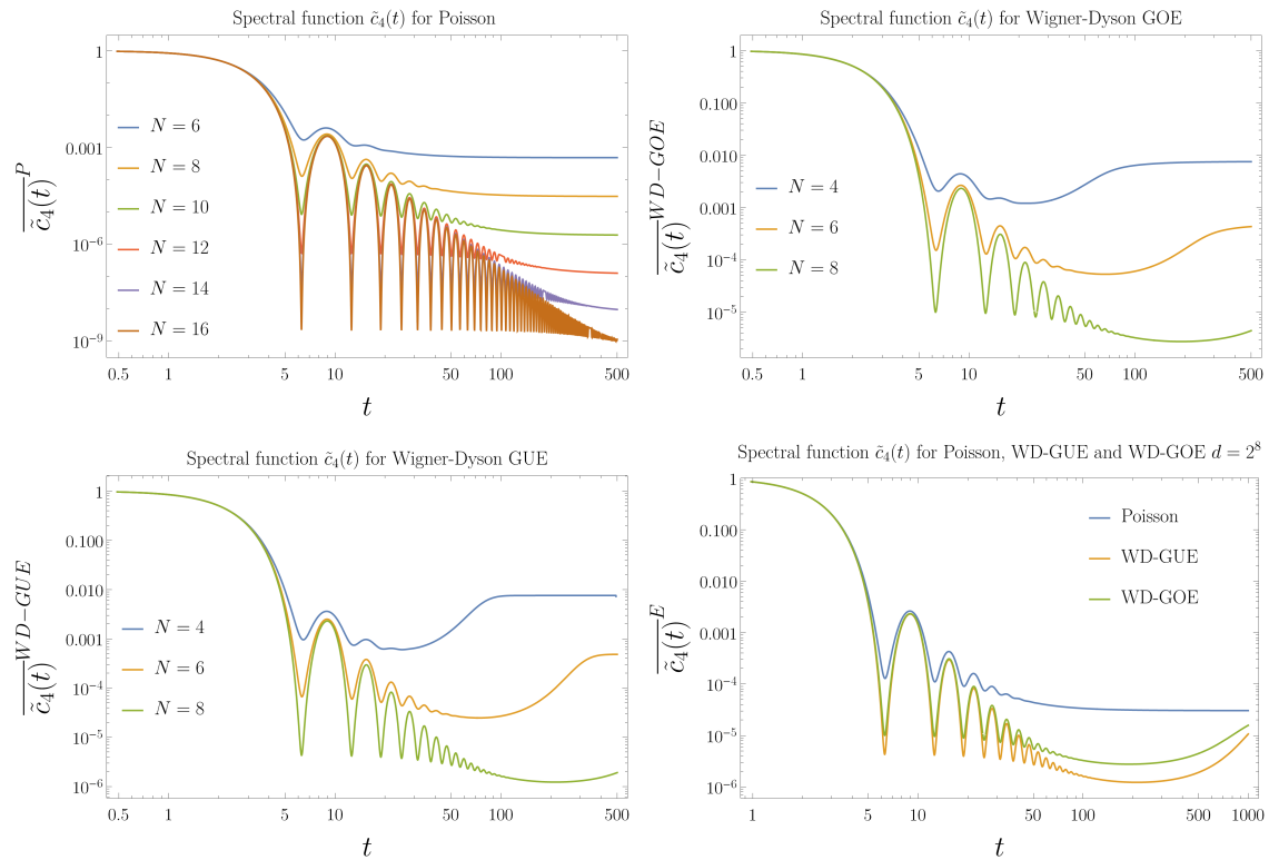
Figure 16: Top-Left : Log Log plot of \tilde{c}_4(t) for Poisson and different system size d = 2^N , N = 6, \dots, 16 . Starting from 1, it reaches the asymptotic value (2d - 1)/d^3 in a time O(d^{1/2}) . Top-Right : Log Log plot of Wigner-Dyson GOE for different system size 2^N , N = 4, 6, 8 . Starting from 1, it goes below the asymptotic value (2d - 1)/d^3 in a time O(d^{1/2}) and reaches the dip O(d^{-2}) in a time O(d^{3/4}) and the asymptotic value in a time O(d) . Bottom-Right : Log Log plot of Wigner-Dyson GUE for different system size 2^N , N = 4, 6, 8 . Starting from 1, it goes below the asymptotic value (2d - 1)/d^3 in a time O(d^{1/2}) and reaches the dip O(d^{-2}) in a time O(d^{3/4}) and the asymptotic value in a time O(d) . Bottom-Left : Comparison between Poisson, Wigner-Dyson from GOE and GUE for d = 2^8 .
