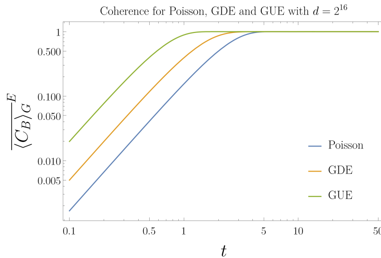
Figure 8: Log-Log plot of \langle C_B(\psi_U) \rangle_G , with \psi = \Pi_j for GUE, Poisson, GDE and d = 2^{16} . We do not observe any scaling difference between the ensembles, they equilibrate in a time O(1) .
