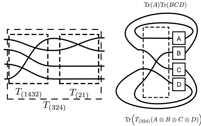
Figure 12: Graphical representation of the swap operator algebra and how the traces work. As a notational note, since the swap operator is defined as T_\sigma = \sum_{ijkl} |\sigma(i)\sigma(j)\sigma(k)\sigma(l)\rangle \langle ijkl| , the permutation group element in the cycle representation is intended to work from the right to the left.
