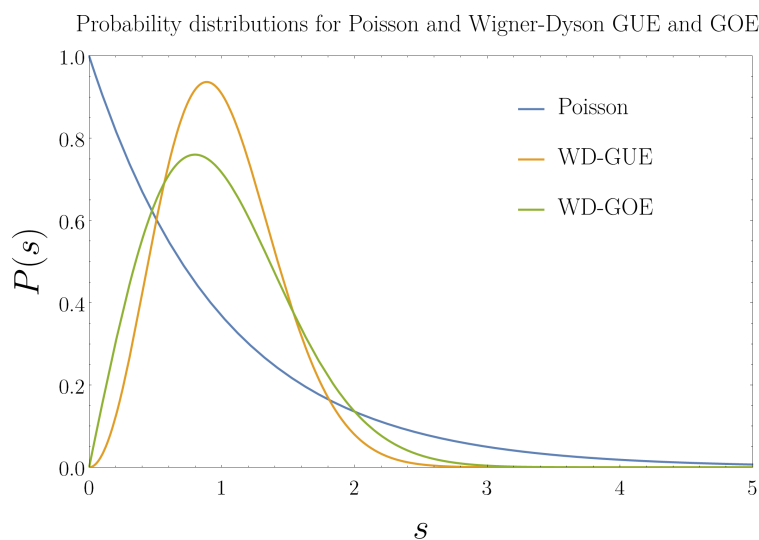
Figure 1: Plot of the nearest level spacing distributions Poisson, Wigner Dyson GUE and GOE reported in Eq. (15).
