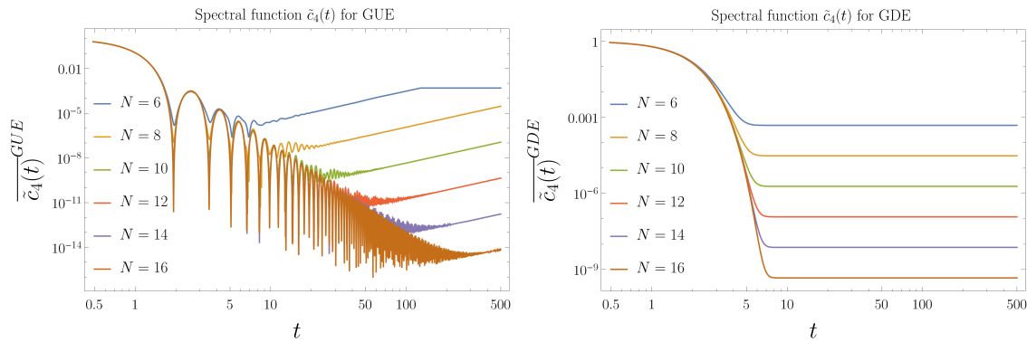
Figure 15: Left : Log Log plot of the normalized spectral function \tilde{c}_4(t) = c_4(t)/d^4 averaged over the GUE ensemble for different system size d = 2^N with N = 6, \dots, 16 . Right : Log Log plot of the rescaled spectral function \tilde{c}_4(t) = c_4(t)/d^4 averaged over the GDE ensemble for different system size d = 2^N with N = 6, \dots, 16
