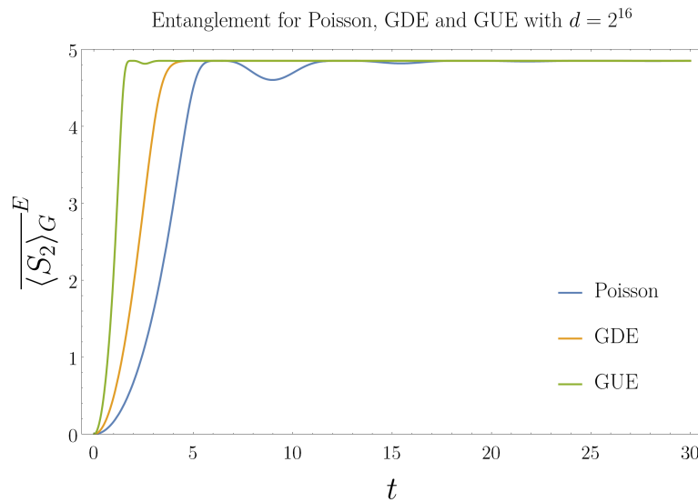
Figure 6: Plot of the r.h.s. of Eq. (45) with \psi_A a pure state for Poisson, GDE and GUE ensembles and d = 2^{16} . GUE and Poisson reveal oscillations before reaching the equilibrium value in a time O(d^{1/12}) and O(d^{1/8}) respectively.
