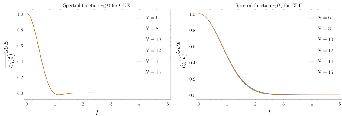
Figure 17: Left : Plot of the normalized \text{Re } c_3(t)^{\text{GUE}} = \text{Re } c_3(t)/d^3 averaged over the GUE ensemble for different system size d = 2^N with N = 6, \dots, 16 . Right : Plot of the rescaled spectral function \tilde{c}_3(t) = c_3(t)/d^3 averaged over the GDE ensemble for different system size d = 2^N with N = 6, \dots, 16 .
