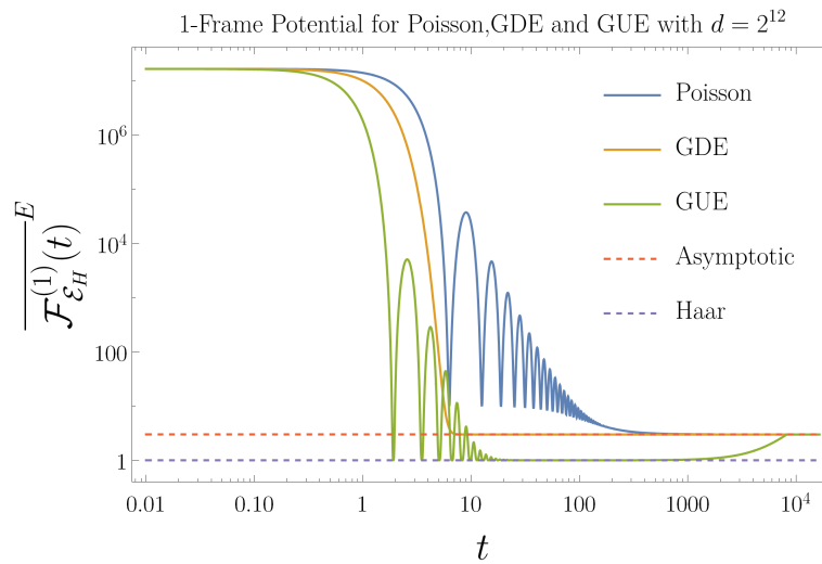
Figure 3: Log-Log plot of the ensemble average of frame potential for the Poisson, GUE and GDE ensemble with system size d = 2^{12} . The dashed lines represent the Haar value 1 and the asymptotic value 3 + O(d^{-1}) . While Poisson and GDE never go below the asymptotic value, GUE stays at the Haar value for the time window t \in [O(d^{1/3}), O(d)] and at late times t \geq O(d) GUE moves away from the Haar value [103] and reaches the asymptotic value. This plot is already shown in [1] and reported here for completeness.
