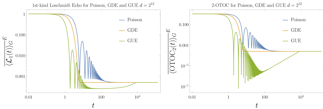
Figure 5: Left : Log Log plot for the Loschmidt-Echo of the first kind (see Eq. (36)) for Poisson, GDE and GUE ensemble and d = 2^{12} . Poisson and GDE being always greater than the asymptotic value 2/d they reach it in a time O(d^{1/2}) and O(\sqrt{\log d}) , while GUE stays at the value 1/d for the whole temporal interval t \in [O(d^{1/3}), O(d)] and then reaches the asymptotic value. Right : Log Log plot of the 2-OTOC see Eq. (43) for Poisson, GUE, GDE ensembles and d = 2^{12} when A is a Pauli operator. The behavior of the 2-OTOC is completely dictated by \tilde{c}_2 : Poisson and GDE reaches the asymptotic value 1/d in a time O(d^{1/2}) and O(\sqrt{\log d}) , while GUE in a time O(d) .
