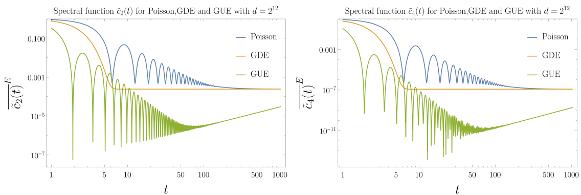
Figure 2: Left : Log-Log plot of the spectral function \overline{\tilde{c}_2(t)}^E for different ensembles E = P , E = GDE and E = GUE for d = 2^{12} . The starting value is 1, while the asymptotic value is d^{-1} . For scalings see Table 2 (Left). Right : Log-Log plot of the spectral function \overline{\tilde{c}_4(t)}^E for different ensemble E = P , E = GDE and E = GUE for d = 2^{12} . The starting value is 1, while the asymptotic value is (2d - 1)d^{-3} . From these plots and from scalings in Table 2(Right) we conclude that c_4(t) distinguishes chaotic from non-chaotic dynamics more efficiently than c_2 .
