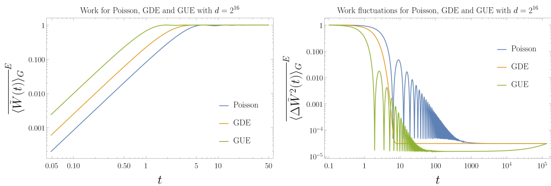
Figure 10: Left : Log-Log Plot of the normalized work in Eq. (73) for Poisson, GDE and GUE and d = 2^{16} . The normalized work starting from 0 at t = 0 and reaches the value 1 in a time O(1) for the three ensembles. Right : Log-Log Plot of the quantity of Eq. (76) for Poisson, GDE, GUE ensembles, where d = 2^{16} and h = 1 . We observe that the timescales are dictated by the timescales of \tilde{c}_2 , cfr. Table 2(Left).
