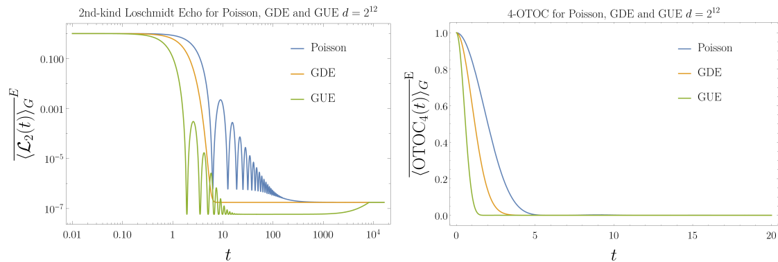
Figure 4: Left : Log-Log plot for the Loschmidt-Echo of the second kind reported in Eq. (36) for Poisson, GDE and GUE ensembles and d = 2^{12} . The Loschmidt-Echo for GDE and Poisson reaches the asymptotic value 3/d^2 after a time O(\sqrt{\log d}) and O(d^{1/2}) respectively, GUE instead equals the offset 1/d^2 for the temporal window t \in [O(d^{1/3}), O(d)] and then reaches the same asymptotic value. Right : Plot of the 4-OTOC for Poisson, GUE, GDE ensemble for d = 2^{12} . The striking feature of the 4-OTOC is the following: while GUE drops to a negative value after a time O(d^{1/3}) , GDE and Poisson never become negative and reach the asymptotic value 1/d^2 in a time O(\sqrt{\log d}) and O(d^{1/2}) respectively.
