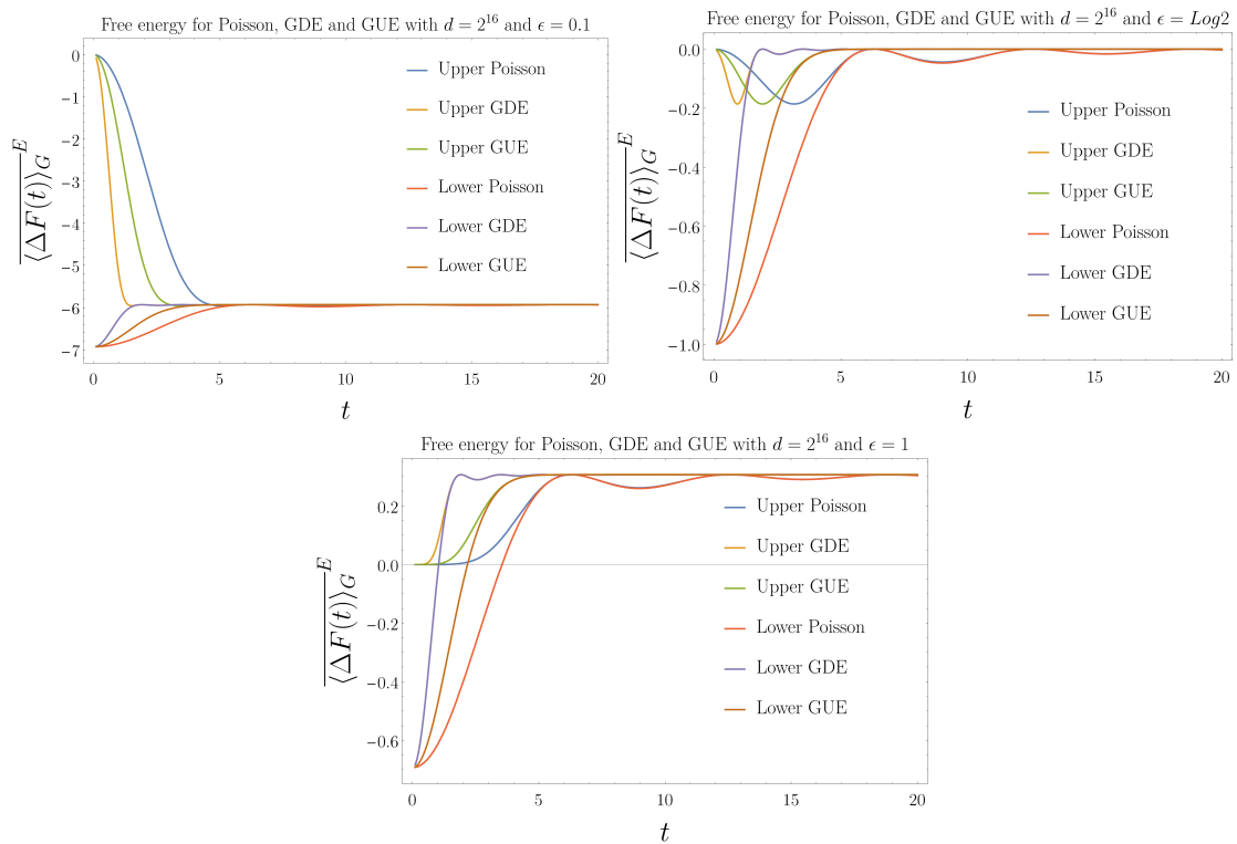
Figure 11: Upper and lower bounds for normalized extractable work \overline{\langle \Delta \mathcal{F} \rangle}_G^E for the Poisson, GUE and GDE ensemble for d = 2^{16} , d_A = 2 and \epsilon = 0.1 (a), \log 2 (b), 1 (c). There is a trade off for \epsilon = \log d_A = \log 2 : the asymptotic extractable work becomes positive, see Eq. (84).
