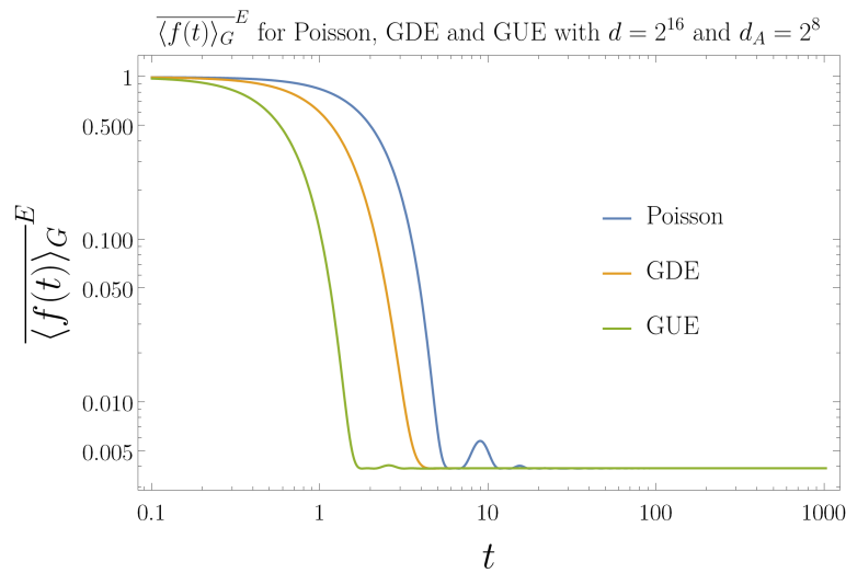
Figure 9: Log-Log plot of \overline{\langle f(t) \rangle_G}^E , see Eq. (69), for d = 2^{16} and d_A = 2^8 averaged over Poisson, GDE and GUE ensemble. The convergence to equilibrium is governed by \tilde{c}_4 ; we observe that GDE, GUE and Poisson equilibrate differently: in a time O(\sqrt{\log d}) , O(d^{1/12}) and O(d^{1/8}) respectively (cfr. Table 2).
