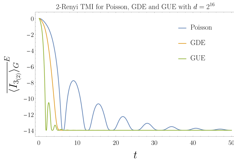
Figure 7: The upper bound for the tripartite mutual information, shown in Eq. (51) for the Poisson, GUE and GDE ensembles for d = 2^{16} . While GDE has no oscillations, GUE and Poisson exhibit oscillations which are reduced with the system size. An analysis of the oscillations is obtained in Eq. (53) and Eq. (54) respectively. This plot is already shown in [1] and reported here for completeness.
