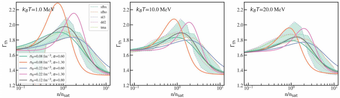
FIG. 2: Effective thermal index for the parameters explored in this work at three different temperatures. From left to right, the panels show \Gamma_{\text{th}} at k_B T = 1, 10 , and 20 MeV; all panels are calculated for matter in neutrino-less \beta -equilibrium. We also show the effective thermal index for a sample of finite-temperature EoSs as dotted lines, for comparison. The green shading is included to visually represent the range of \Gamma_{\text{th}} values spanned by the realistic EoS tables. All sets of M^* -parameters confirm that \Gamma_{\text{th}} indeed depends on the density. The degree of density-dependence is directly governed by the parameter \alpha , while the density at which \Gamma_{\text{th}} begins to vary is determined by the parameter n_0 .
