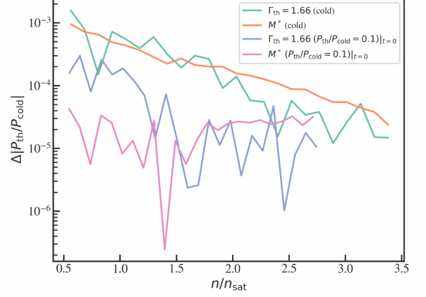
FIG. 11: Total change in the characteristic thermal pressure at each density, between the initial and final time steps (i.e., |P_{\text{th}}/P_{\text{cold}}(t=0) - P_{\text{th}}/P_{\text{cold}}(5t_{\text{dyn}})| ). All profiles correspond to the highest-resolution evolutions. Both the hybrid and M^* evolutions maintain the initial thermal profile to within \lesssim 1 part in 10^3 at supranuclear densities, for both zero- and finite-temperature initial data.
