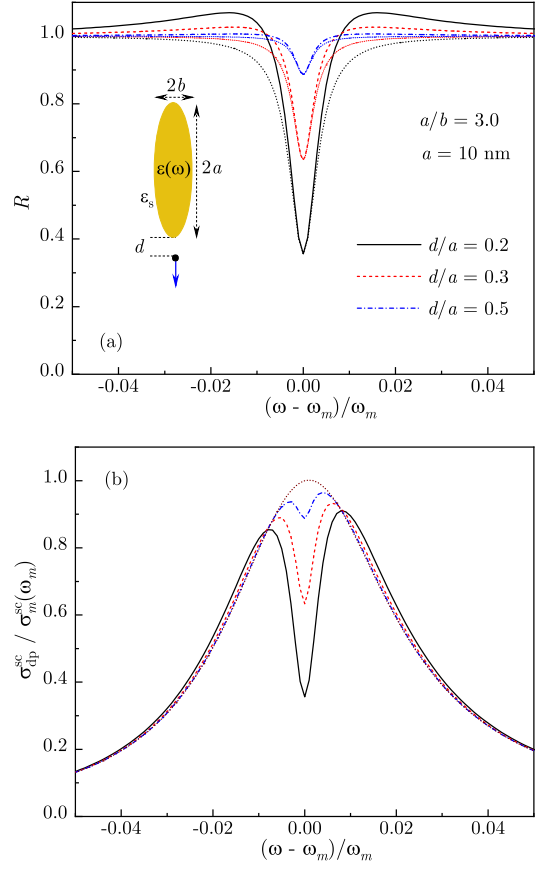
FIG. 2. (a) The ExIT function R(\omega) , given by Eq. (35), and its asymptotic expression (dotted lines), given by Eq. (37), are shown for a QE near the tip of Au nanorod with aspect ratio a/b = 3.0 and length 2a = 20 nm at distances d/a = 0.5, 0.3 , and 0.2 . (b) Normalized scattering cross-section in the dressed plasmon approximation is shown for the same system parameters. Dotted line is the plasmon band. All curves are calculated for \omega_e = \omega_m . Inset: Schematics of a QE situated at a distance d from the tip of Au nanorod in water for QE dipole moment oriented along the nanorod axis.
