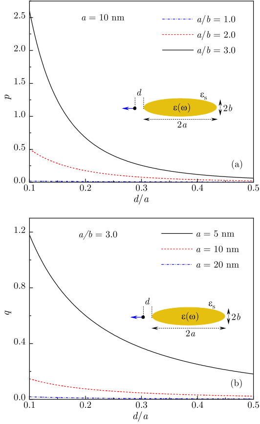
FIG. 1. (a) The ExIT parameter p is plotted against the QE distance d to the tip of Au nanorod of length 2a = 20 nm placed for different values of aspect ratio a/b = 1.0, 2.0 and 3.0 . (b) The Fano parameter q is plotted against the distance d at nanorod aspect ratio a/b = 3.0 for different values of nanorod length 2a = 40 nm, 20 nm and 10 nm. Inset: Schematics of a QE situated at a distance d from the tip of Au nanorod in water for QE dipole moment oriented along the nanorod axis.
