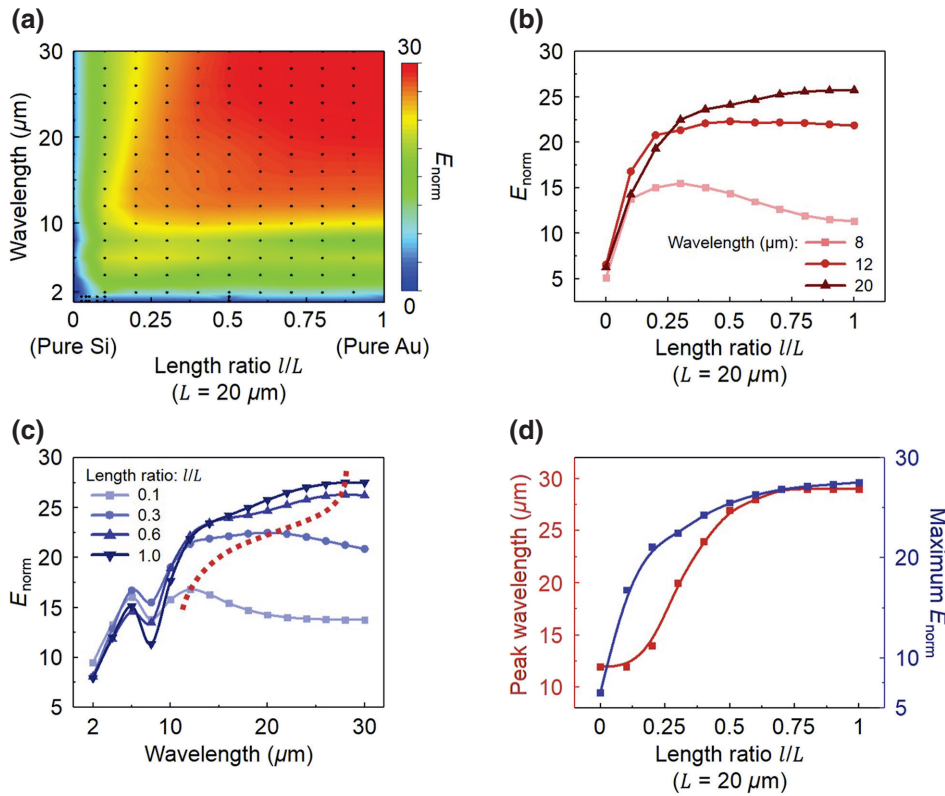
FIG. 2. Simulation of the CLE in near- and mid-IR range. (a) The near-field enhancement mapping for different length ratios with L fixed at 20 \mu\text{m} . The E_{\text{norm}} is calculated at 20 nm above the tip apex. (b) The horizontal line cuts of the mapping, showing the E_{\text{norm}} as a function of length ratio with different illuminating light wavelengths. (c) The vertical line cuts of the mapping, showing the E_{\text{norm}} as a function of illuminating light wavelength with different length ratios. The red dotted line marks the maximum E_{\text{norm}} point for each length ratio. (d) The wavelength and maximum E_{\text{norm}} of different length ratios corresponding to the red dotted line shown in (c), which is supplemented by a finer scan with smaller wavelength steps (Fig. S2 in the Supplemental Material [17]).
