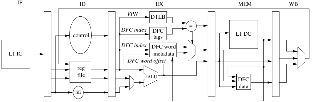
Fig. 7. Modified Datapath to Support Guaranteed DFC Hits
