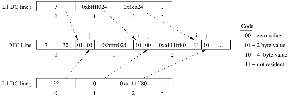
Fig. 5. Example of Line Sharing and Data Packing
