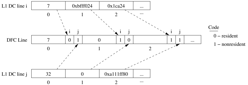
Fig. 4. Example of Line Sharing
