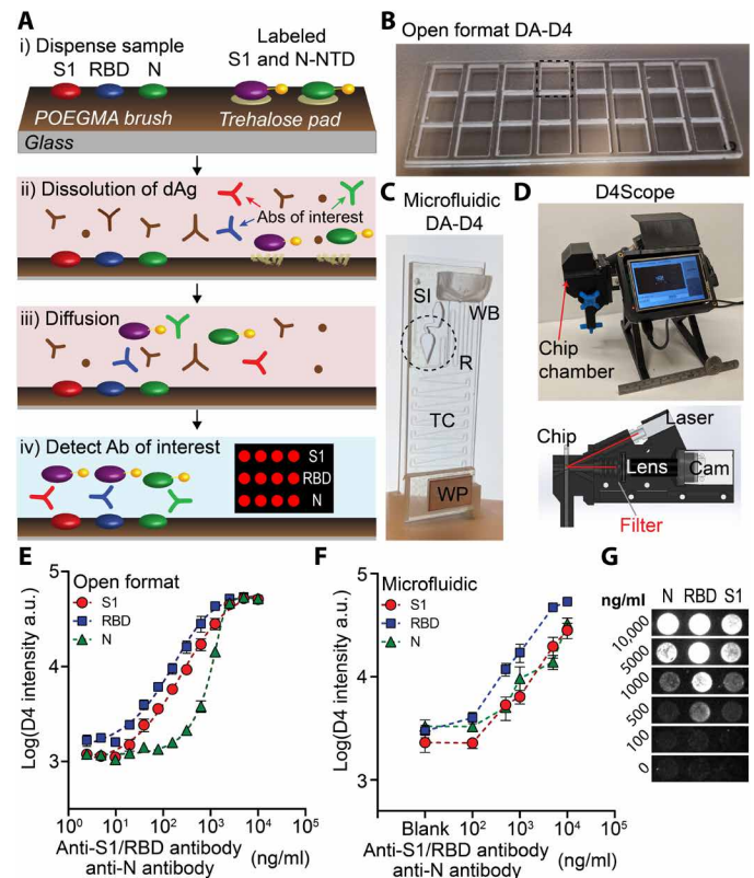
Fig. 1. DA-D4 POCT schematic and analytical validation. (A) DA-D4 assay chip schematic. S1, RBD, and N capture antigens and fluorescently labeled S1 and N-NTD detection antigens (dAg) are inkjet-printed onto a POEGMA substrate. When a sample is added, dAg are liberated from the surface owing to the dissolution of the underlying trehalose pad. Antibodies targeting each viral antigen then bridge the capture antigens to the dAg, resulting in a fluorescence signal that scales with antibody concentration. (B) Open-format DA-D4 with 24 individual assays. (C) Microfluidic DA-D4. Sample is added to the sample inlet (SI), filling the reaction chamber (R) that contains the assay reagents. Wash buffer (WB) is added to the WB reservoir, which chases the sample through the microfluidic cassette. The timing channel (TC) sets the incubation time. All liquid is eventually soaked up by the wicking pad (WP) after the incubation process. The size is that of a standard microscope slide. (D) D4Scope and cut-away view of the optical path. The microfluidic flow cell is inserted on the left and pressing a button automates laser excitation, camera exposure, and data output. (E) Analytical validation of the open-format DA-D4. Antibodies targeting each antigen were spiked into undiluted human serum and incubated for 30 min. Each data point represents the average of three independent runs, and the error bars represent the SEM. a.u., arbitrary units. (F) Analytical validation of microfluidic DA-D4. Each data point for an antigen represents the average of four independent microfluidic flow cells and error bars represent the SEM. (G) Representative D4 spots shown for each dose. Photo credit for (B) to (D): David S. Kinnamon, Duke University.
