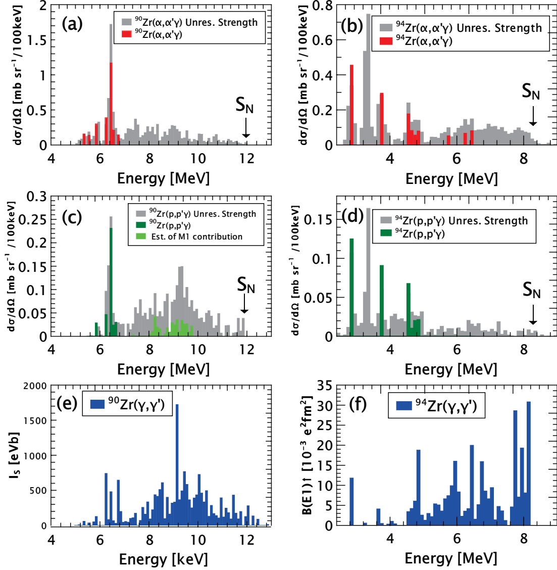
Figure 2: Cross section for the excitation of dipole states from different reaction types for the nuclei ^{90}\text{Zr} and ^{94}\text{Zr} . Panels (a) and (b) are for the (\alpha, \alpha')\gamma reaction at 130 MeV, panels (c) and (d) are for the (p, p')\gamma reaction at 80 MeV, while panels (e) and (f) show (\gamma, \gamma') measurements from references [15] and [16]. The coloured bars correspond to discrete transitions while the grey bars correspond to the continuum regions in the present measurements. In panel (c) the estimated contribution from 1^+ states obtained using the measured M1 strength from [17] is shown in the grey area with light green bars.
