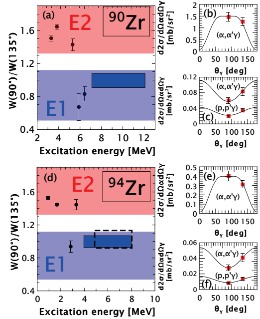
Figure 1: The ratio of the measured yields at 90° and 135° for several transitions and the continuum regions (marked by horizontal blue bars) for ^{90}\text{Zr} (panel(a)) and ^{94}\text{Zr} (panel (d)) measured with the (\alpha, \alpha'\gamma) reaction at 130 MeV. In both frames, the coloured regions refer to E2 (in red) and E1 (in blue) transitions types. The vertical size of the dark blue regions represents the statistical uncertainty related to the integral of counts. In panel (d) the rectangular region limited by dashed lines does not include the discrete transitions between 4.5 and 4.9 MeV. The measured and predicted \gamma angular correlations for selected discrete lines are shown panels (b),(c),(e),(f). The predictions were obtained with DWBA calculations. Panel (b) is for the 2186 keV E2 transition of ^{90}\text{Zr} and panel (c) is for the 6425 keV E1 transition of ^{90}\text{Zr} . Panel (e) is for the 919 keV E2 transition of ^{94}\text{Zr} and panel (f) is for the 2846 keV E1 transition of ^{94}\text{Zr} . The angular correlations for the (p, p'\gamma) reaction, are characterised by a smaller anisotropy.
