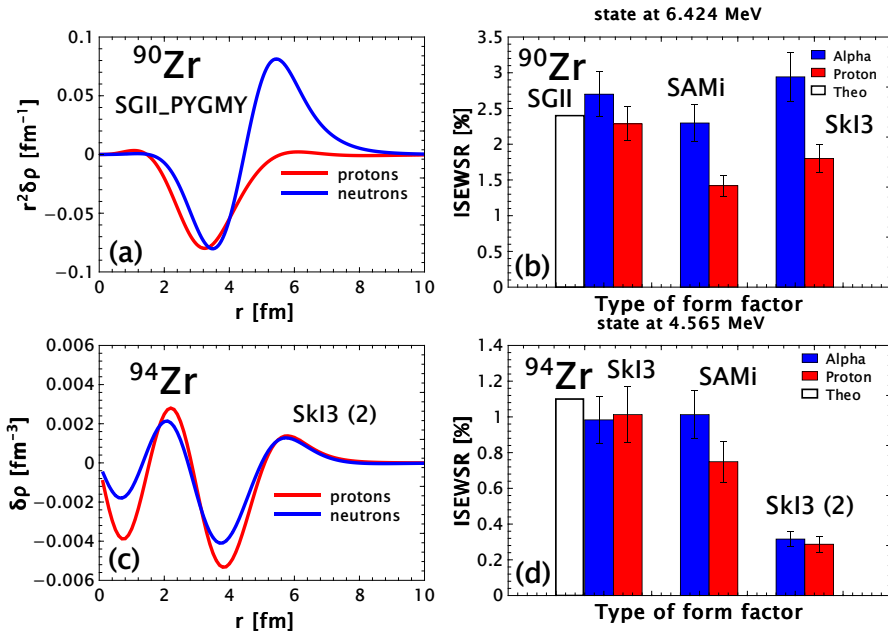
Figure 3: Panels (a) and (c) show two predictions of the transition densities, one for the nucleus 90 Zr - typical of a pygmy dipole state - calculated with a SGII interaction (top left panel) and one for the nucleus 94 Zr - with no isospin mixing at the nuclear surface - calculated with a SkI3 interaction (bottom left panel) and indicated as SkI3(2). Panels (b) and (d) show the fraction of the ISEWSR strength deduced by comparing the data from \alpha (blue bars) and proton (red bars) scattering with DWBA calculations using form factors calculated using transition densities obtained with different interaction within the EDF+RPA approach. Panel (b) refers to the 6424 keV state in 90 Zr and panel (d) is for the 4565 keV state in 94 Zr. For the SGII interaction for 90 Zr and the SkI3 interaction for 94 Zr the theoretical values of the ISEWSR strength are also shown with the empty bars. The bars denoted with SkI3(2) were obtained by using the transition densities on the bottom left panel while the ones indicated with SkI3 were obtained with transition densities that have a shape similar to the ones on the upper left panel.
