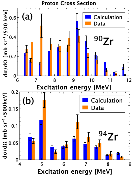
Figure 4: The cross section measured with proton inelastic scattering at 80 MeV (integrated over a bin 0.5 MeV wide and in mb/sr) is shown with orange bars and the corresponding prediction, including as strength that determined by the (\alpha, \alpha') data, is shown with blue bars. Panel (a) is for the ^{90}\text{Zr} nucleus and panel (b) for the ^{94}\text{Zr} nucleus. The predictions are based, as described in the text, on DWBA calculations using values of the E1 EWSR strengths that were deduced from fitting of \alpha scattering data of this work.
