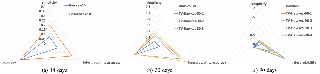
Fig. 2: Model comparison using IMPD dataset. The three axes in the radar chart are simplicity, interpretability, and accuracy. From left to right, the charts represent models with window sizes of 14, 30, and 90 days.
