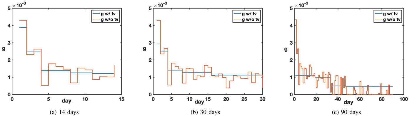
Fig. 3: Estimated kernels using the IMPD data. From left to right, the window sizes are 14, 30, and 90 days; \mu_{TV} = 1 \times 1e-4 , 3 \times 1e-4 , and 1.2 \times 1e-3 . Blue curve: TV-Hawkes; Red curve: Hawkes.
