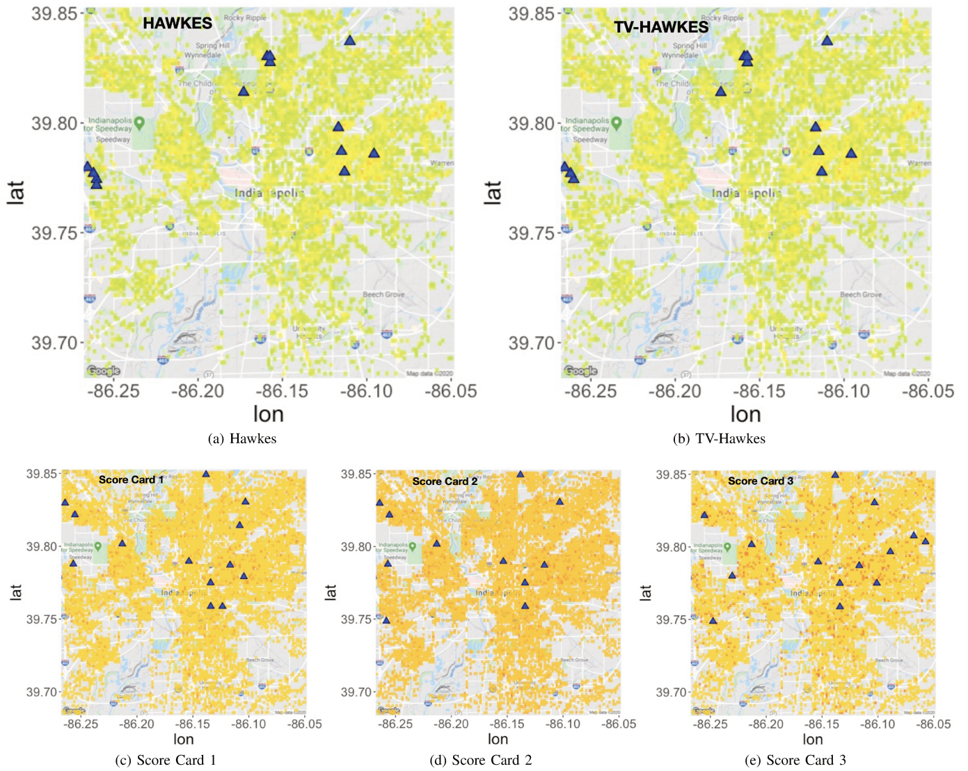
Fig. 4: Intensity for a random day (from the test set). Top left: intensity estimated using regular Hawkes process; Top right: intensity estimated using TV-Hawkes process (30-day window). Bottom: from left to right, intensity estimated using Score Card 1, 2, and 3. The grid cells are colored based on the fourth root of intensity (strong: red, medium: yellow, weak: green). The blue triangles represent the top-20 forecasted cells. The cells with zero intensity are set as transparent.
