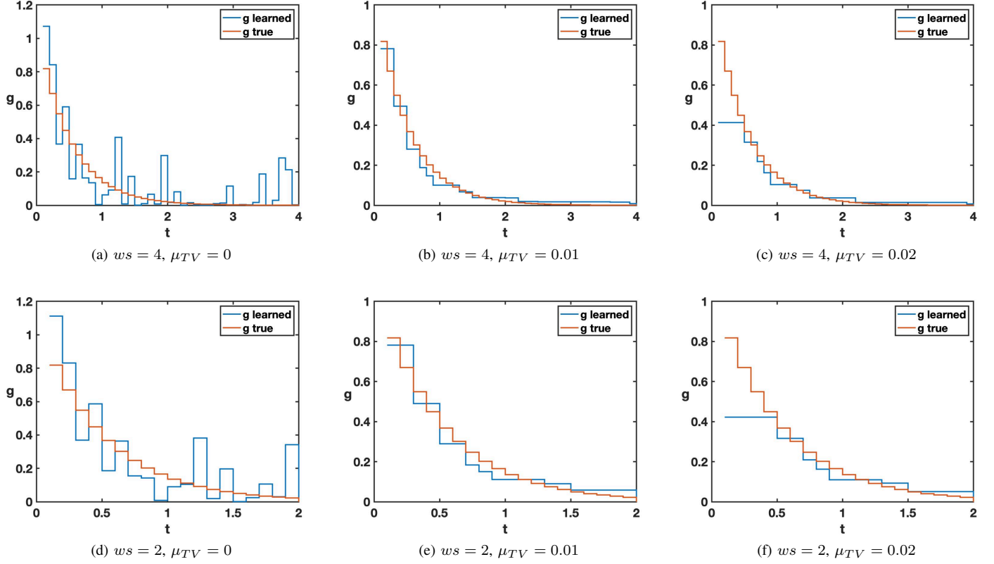
Fig. 1: Synthetic experiments. Hawkes process with an exponential kernel. Orange curve: true kernel; Blue curve: estimated kernel. Top: kernel is truncated at 4; Bottom: kernel is truncated at 2. From left to right, the figures represent Hawkes model, Hawkes-tv with \mu_{TV} = 0.01 , and 0.02.
