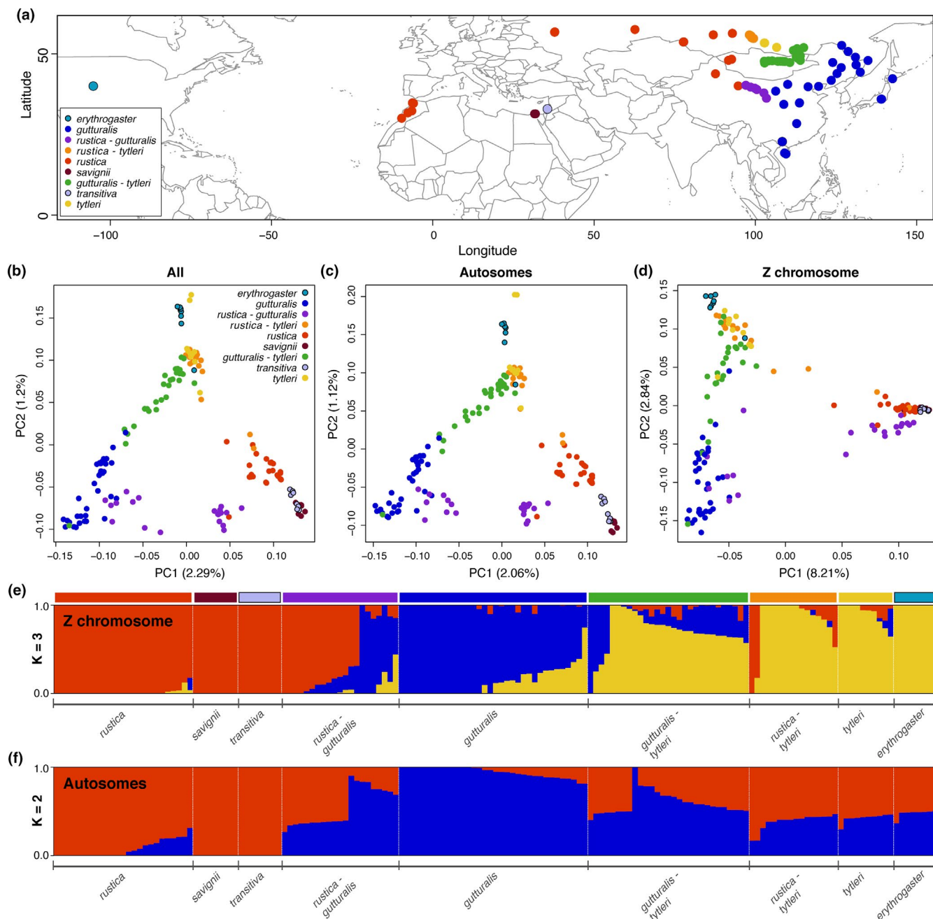
FIGURE 4 PCA and population structure analyses. (a) Map of sampled localities throughout the barn swallow breeding range. The colours of points represent subspecies and hybrid zones and correspond with the colours used in the PCA results in (b)–(d). (b) Results of PCAs for all SNPs. (c) PCA results for autosome-only SNPs. (d) PCA results for Z chromosome-only SNPs. (e) Inferred ancestry assignments from ADMIXTURE analysis of Z-linked SNPs under a best-supported K = 3 model. Each vertical bar represents the probability of assignment of an individual to one or more genetic clusters. (f) Ancestry assignments from ADMIXTURE analysis of autosomal SNPs under a K = 2 model. Coloured horizontal bars above the ancestry plots correspond to colours used in (a)–(d) for subspecies and hybrid zones [Colour figure can be viewed at wileyonlinelibrary.com ]
