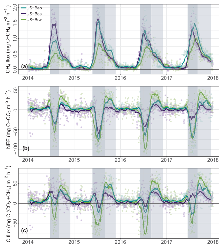
Figure 3. Carbon flux (daily average) of (a) \text{CH}_4 , (b) \text{CO}_2 and (c) \text{CO}_2 + \text{CH}_4 (with \text{CH}_4 expressed as \text{CO}_2 -eq based on warming potential) at the three EC sites. The darker shaded portion represents the growing season, while the lighter shaded portion represents the zero-curtain period.
