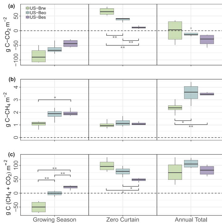
Figure 4. Seasonal and yearly budgetary contributions of (a) \text{CO}_2 , (b) \text{CH}_4 and (c) \text{CO}_2 + \text{CH}_4 (expressed as \text{CO}_2 -equivalent based on warming potential) at the three EC sites from the growing season, zero-curtain period, and yearly total (* p < 0.05 ; ** p < 0.01 ).
