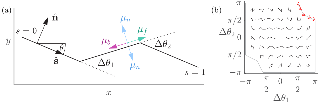
FIG. 2. (a) Schematic diagram of a three-link body with changes in angles \Delta\theta_1 (here positive) and \Delta\theta_2 (here negative) between the links. The body is parametrized by arc length s (nondimensionalized by body length) at an instant in time. The tangent angle and the unit vectors tangent and normal to the curve at a point are labeled. Vectors representing forward, backward, and normal velocities are shown with the corresponding friction coefficients \mu_f , \mu_b , and \mu_n . (b) Examples of body shapes in the (\Delta\theta_1, \Delta\theta_2) -plane. Shapes that do not self-intersect are shown in black; a few shapes at the threshold of self-intersection are shown in red.
