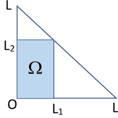
Fig. 1 The domain D of our algebraic curves is contained inside the rectangle \Omega = [0, L_1] \times [0, L_2] , which we embed inside a triangle with vertices (0, 0) , (L, 0) , (0, L) .
