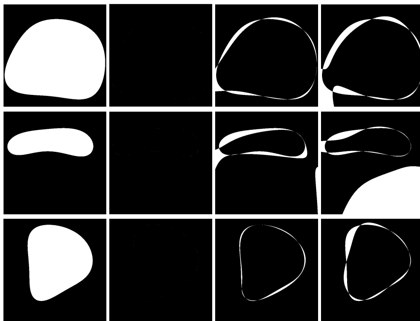
Fig. 7 Sensitivity of reconstruction to sampling kernel. Algebraic shapes of size of degree four (column 1) were reconstructed using our BMR algorithm from 32 \times 32 noisy samples with \text{SNR} = 100 dB using different sampling kernels. Absolute error of reconstruction using B-spline, Daubechies and pseudospline kernels is shown in columns 2, 3 and 4 respectively.
