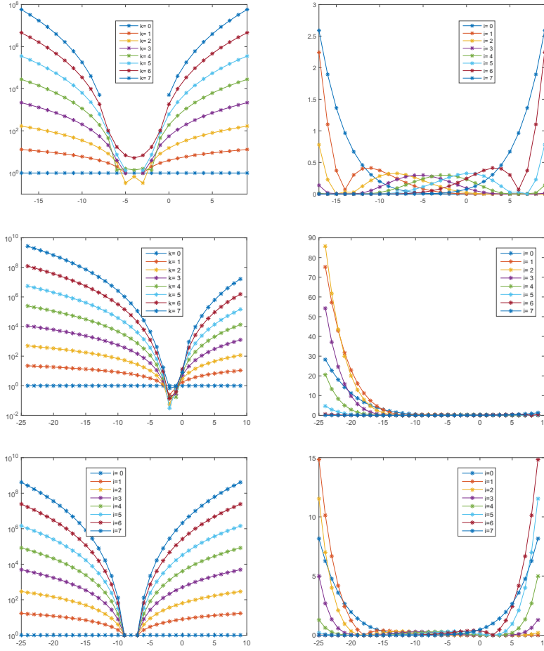
Fig. 2 Behaviour of the coefficients generating the monomials x^i (left) and the Bernstein polynomials B_i^7 (right), for i = 0, \dots, 7 , when the kernel \varphi is the B-spline of order 8 (top), the Daubechies scaling function associated to 7 vanishing moments (middle) and the dual pseudospline of order 8
