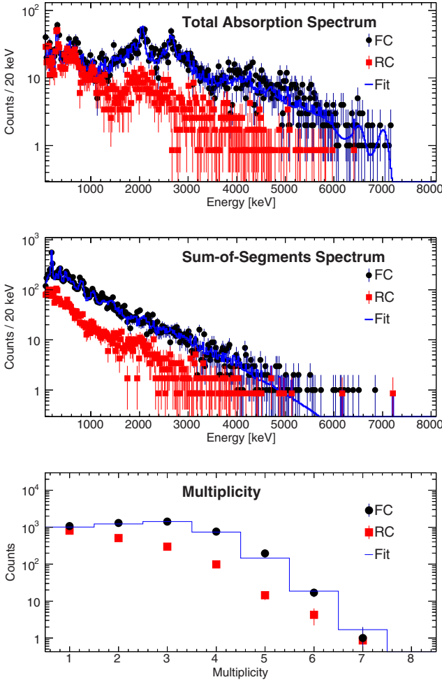
FIG. 4. The best fit to the data for the \beta decay of ^{104m}\text{Nb} . Only three of the nine fitted spectra are shown. The best fit are the blue lines. The RC spectra are in red (square markers). The FC spectra are in black (circular markers). The RC spectra are generally below the FC spectra which indicates that the FC spectra are not completely dominated by RC. FC is dominated by random correlations below 1 MeV.
