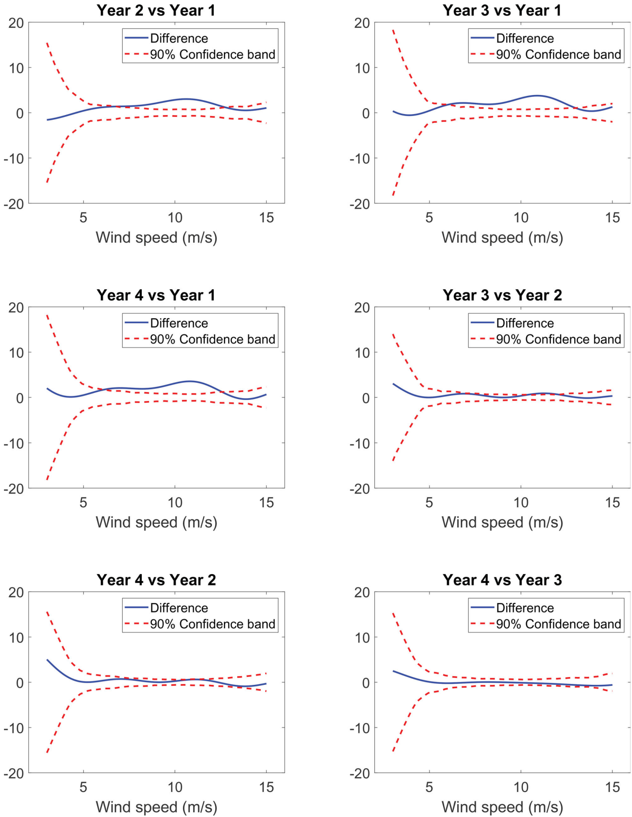
Figure 4. Difference in curves vs wind speed for WT1.
