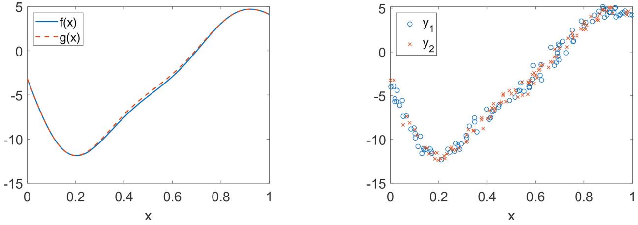
Figure 1. Plots for GP sample. Left panel: f(x) and its perturbation, g(x) ; Right panel: Noisy realizations from f(x) and g(x) .
