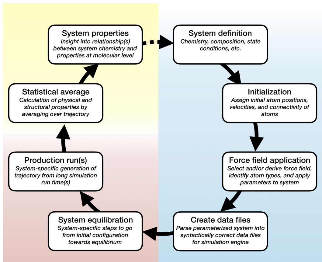
FIGURE 1 Typical steps involved in performing a molecular simulation. If all steps are scriptable, the entire process can be encased in a loop over hundreds or thousands of chemistry, composition, and/or state conditions combinations to enable screening for desirable properties. Background colors refer to: initialization steps (blue), simulation run time steps (red), and system analysis steps (yellow)
