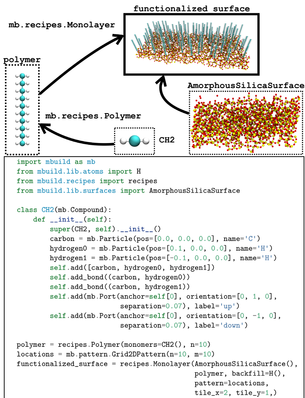
FIGURE 2 Python script that uses mBuild to define a class for a –CH 2 – group, create a polymer composed of multiple –CH 2 – groups, and connects copies of this polymer to a surface. Note for simplicity, the terminal –CH 3 group is not shown. Additional mBuild tutorials and example scripts are available online at https://github.com/mosdef-hub/mbuild_tutorials
