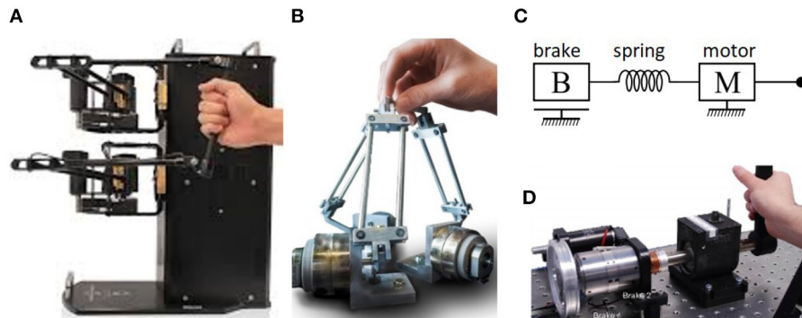
FIGURE 1 | Different actuation techniques for haptic devices. (A) is a traditional haptic device (HD 2 from Quanser Inc) with electric motors [reproduced from Quanser (2020) with permission from Quanser Inc.], (B) employs a set of three rheological brakes (Lacki and Rossa, 2020) [reproduced from Lacki and Rossa (2020) with permission from IEEE], in (C) a brake-motor-spring drive is proposed as an alternative to passive actuators (Conti and Oussama, 2009), and arrangement (D) has two unidirectional brakes coupled with a motor (Rossa et al., 2014) [reproduced from Rossa et al. (2014) with permission from IEEE].
