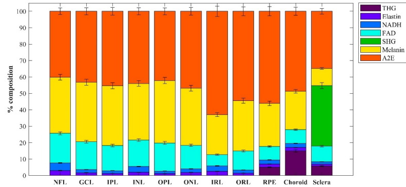
Figure 2. Quantitative analysis of a retina done by super-phasor unmixing in the wavelength domain. Reproduced from Ref 4 with permission
