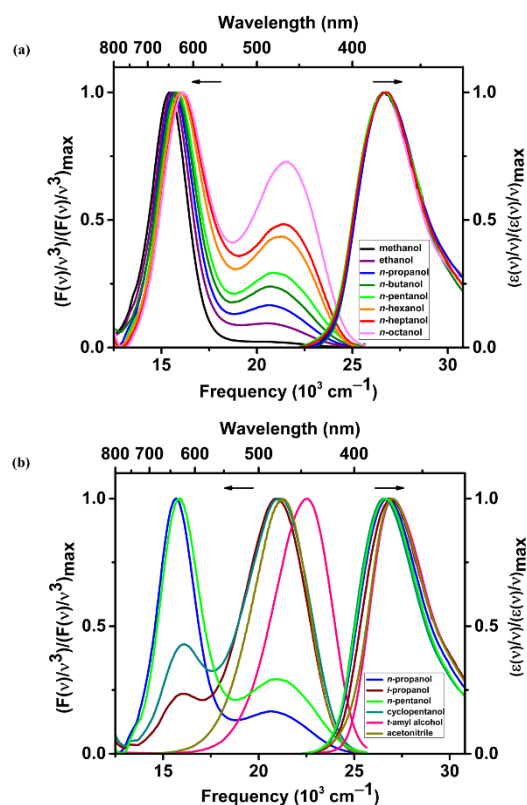
Fig. 2 Steady-state absorption and fluorescence spectra of FRO-SB in alcohols. (a) The normalized absorption and emission spectra of FRO-SB in primary alcohols from methanol to n -octanol. (b) The absorption and emission spectra of FRO-SB in various solvents to compare steric hindrance. The long wavelength emission near 630 nm ( \sim 15,870\text{ cm}^{-1} ) corresponds to FRO-HSB + * , while the short wavelength emission near 460 nm ( \sim 21,740\text{ cm}^{-1} ) corresponds to FRO-SB * .
