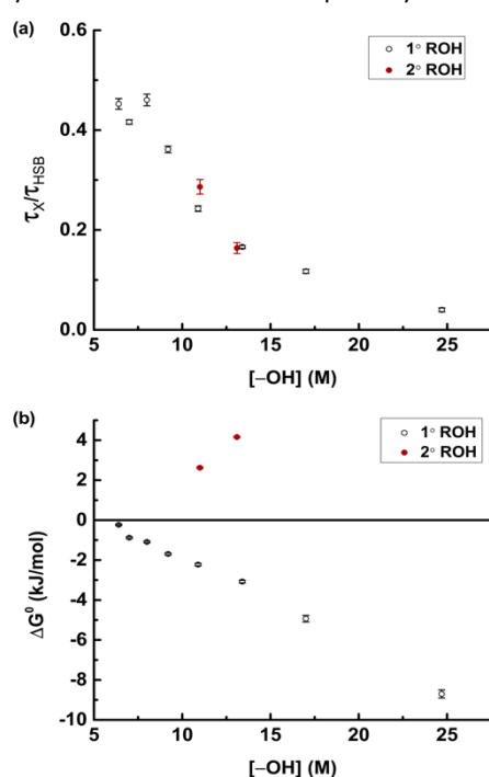
Fig. 6 Trends in dynamics and free energy as a function of relative [-OH] . (a) The ratio of the time constants \tau_X and \tau_{HSB} is plotted as a function of relative [-OH] . (b) \Delta G^\circ for proton abstraction obtained from the ratio of FRO-SB^* to FRO-HSB^{+*} emission as a function of relative [-OH] . We note good agreement between the time-resolved and the steady-state data for the linear alcohols.
