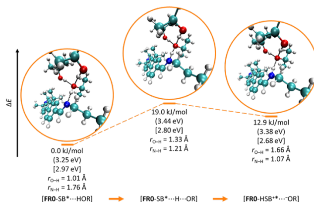
Fig. 11 Snapshots of the proton abstraction process from i -propanol. The SMD/CAM-B3LYP/6-31+G* optimized geometries of the [FRO-SB*...HOR] reactant, [FRO-SB*...H...OR] transition state, and [FRO-HSB*...OR] product of the ESPT process between FRO-SB in its S_1 electronic state and three i -propanol molecules (see the ESI† for the computational details). The \Delta E values in kJ/mol are given relative to the reactant energy. The energies inside parentheses, in eV, are given relative to the [FRO-SB*...HOR] minimum in the ground electronic state S_0 , while those inside square brackets correspond to the S_0 \rightarrow S_1 vertical transitions at each respective geometry. The r_{O-H} and r_{N-H} distances at each geometry represent the internuclear separations between the proton being transferred and the oxygen of i -propanol and the imine nitrogen of FRO-SB , respectively.
