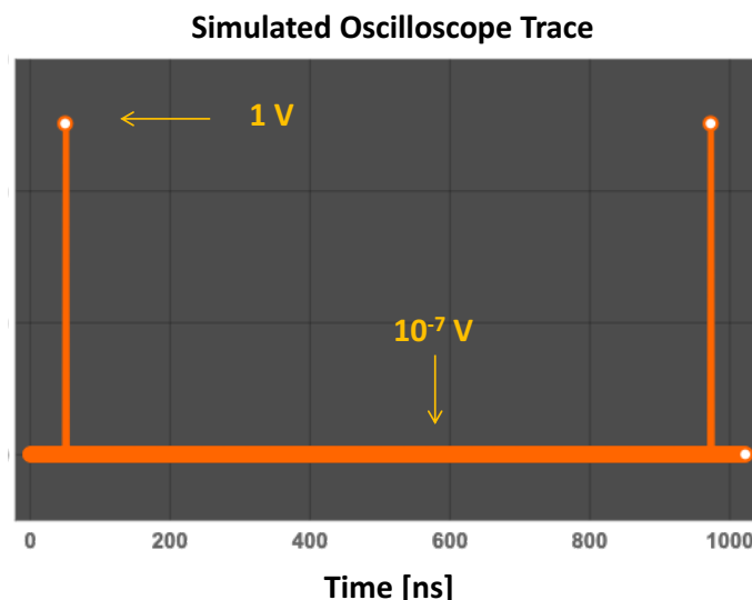
Figure 1. Graphic illustrating the simulated oscilloscope train for a 1 MHz repetition rate 100 W laser with a power figure of merit of 0.9. The vertical corresponds to the number of photons per bin size (here 1 ns), while the horizontal axis illustrates time, here in nanoseconds. Given the 0.9 power figure of merit, we know that 10% of the power is distributed in the time between the pulses. However, that time is so long that the number of photons is too small to be seen on a linear scale.
