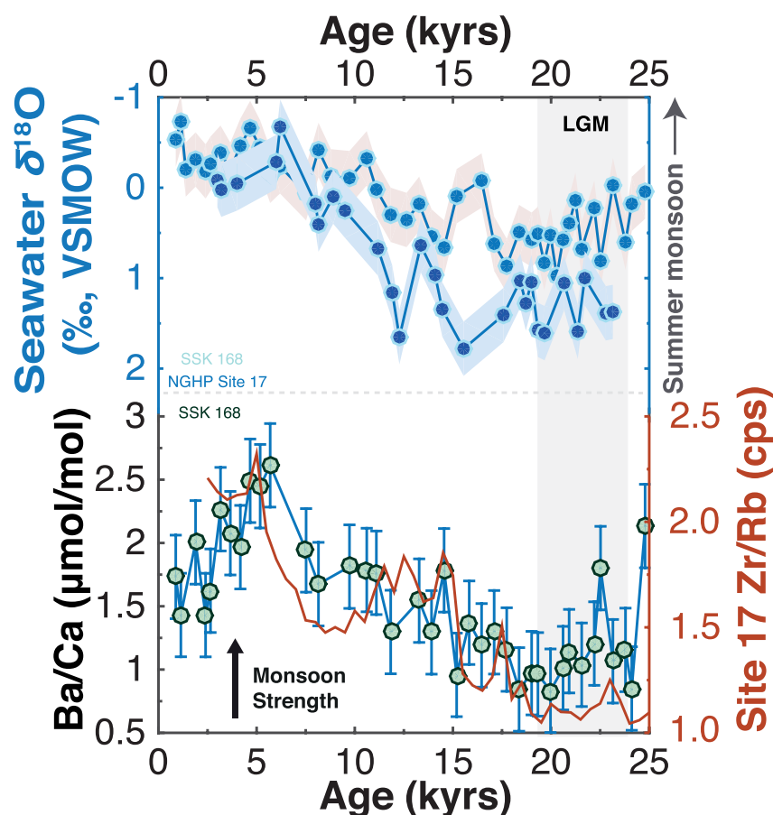
Figure 9. Comparison between Zr/Rb ratios (cps) with monsoon precipitation intensity changes inferred from reconstructed \delta^{18}\text{O}_{\text{sw}} time series from cores SSK 168 (Gebregiorgis et al., 2016) and NGHP Site 17 (Gebregiorgis et al., 2018), and Ba/Ca records from core SSK 168 (Gebregiorgis et al., 2016) in the Andaman Sea over the last ~25 kyr. Envelope in upper figure denotes uncertainty in \delta^{18}\text{O}_{\text{sw}} reconstructions. Inverted triangles in red and black show radiocarbon dates for core sites NGHP17 and SK168, respectively.
