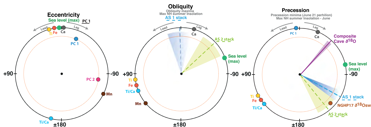
Figure 13. Phase wheels summarizing the response of the two PCs and major contributing elements and ratios at the orbital eccentricity (100 kyr), obliquity (41 kyr), and precession (23 kyr). The precession index is defined as \Delta \sin \omega where \omega is the longitude of the perihelion measured from the moving vernal point and \epsilon is the eccentricity of Earth's orbit around the Sun (Berger & Loutre, 1997; Laskar et al., 1993). Obliquity is the axial tilt of Earth's rotation axis with respect to the orbital plane. In the phase wheel representation the 12 o'clock position is set to precession minima (P min; \omega = 90^\circ , 21 June perihelion) and obliquity maxima (O max), respectively. Negative/positive phases are measured in the clockwise/anticlockwise direction and represent phase lags/leads relative to P min or O max. Published records plotted (with shaded phase estimate errors) are the Arabian Sea summer monsoon stacks AS1 (Caley et al., 2011) and AS2 (Clemens & Prell, 2003), the Chinese Sanbao-Hulu cave \delta^{18}\text{O} composite (Cheng et al., 2016). Ice volume (IV) corrected \delta^{18}\text{O}_{\text{sw}} (a measure of surface water salinity) from NGHP Site 17 (Gebregiorgis et al., 2018). The orange circle denotes 80% coherence.
