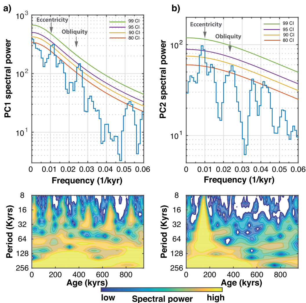
Figure 12. a) Redfit spectral analysis of the a) PC1 and b) PC2 time series. Continuous wavelet transform of the PCs are also shown in the same order.
