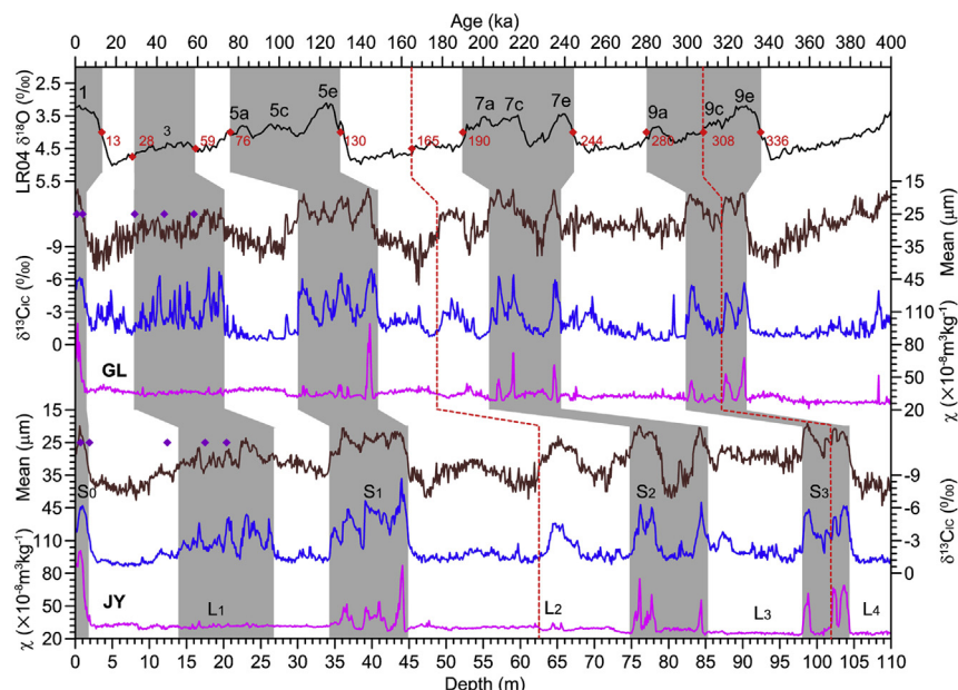
Fig. 2. Variations of magnetic susceptibility ( \chi , pink), mean grain size (brown) and \delta^{13}\text{C}_{\text{IC}} (blue) of the GL and JY sections, and their correlation with benthic \delta^{18}\text{O} stack (black, Lisiecki and Raymo, 2005). Red diamonds indicate ages derived from tie points linking rapid changes in mean grain size with the boundaries of marine isotope stages (MIS) recorded by the benthic \delta^{18}\text{O} record. Red dashed lines denote two additional ages derived within MIS 6 and 9, respectively. Purple diamonds are the optically stimulated luminescence dates (Sun et al., 2012b). (For interpretation of the references to color in this figure legend, the reader is referred to the web version of this article.)
