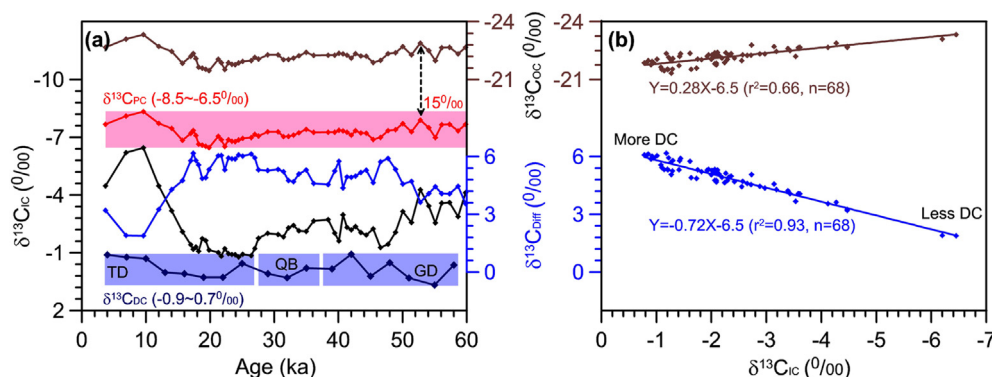
Fig. 5. (a) Glacial–interglacial variations of \delta^{13}C_{OC} , \delta^{13}C_{PC} , \delta^{13}C_{Diff} , and \delta^{13}C_{IC} , and their comparison with the \delta^{13}C_{DC} results; (b) Comparison of \delta^{13}C_{IC} with \delta^{13}C_{Diff} and \delta^{13}C_{OC} . \delta^{13}C_{PC} is estimated from \delta^{13}C_{OC} by subtracting 15‰ (Cerling et al., 1989; Liu et al., 2011). \delta^{13}C_{Diff} denotes the carbon isotopic difference between \delta^{13}C_{PC} and \delta^{13}C_{IC} , with large difference corresponding to more proportion of detrital carbonate (DC).
