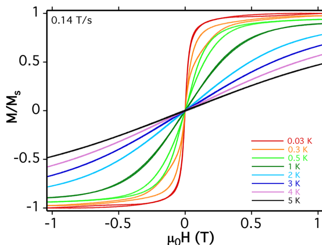
Figure 4. Field dependence of the normalized magnetization of \mathbf{I}_{\text{Mn}} in the temperature range 0.03–5 K at field sweep rate of 0.14 T s −1 .
