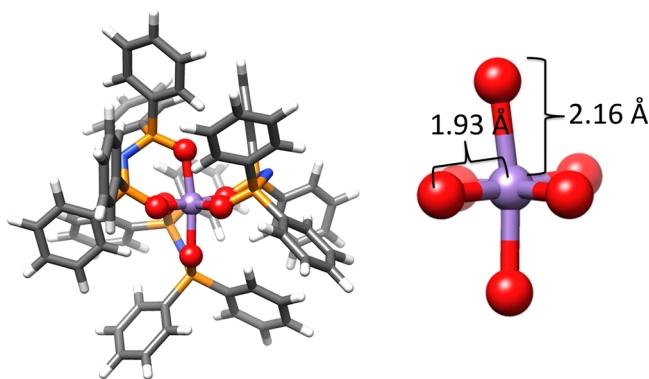
Figure 1. Molecular structure of \mathbf{1}_{\text{Mn}} . 28,41 Color code: Mn, purple; O, red; P, orange; N, blue; C, gray; H, white.
