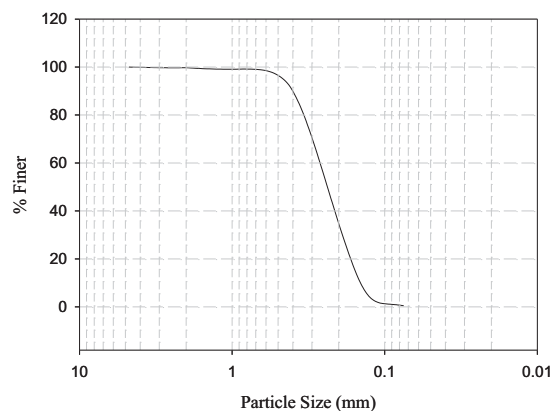
Figure 3. Soil particle size distribution from sieving analysis.
