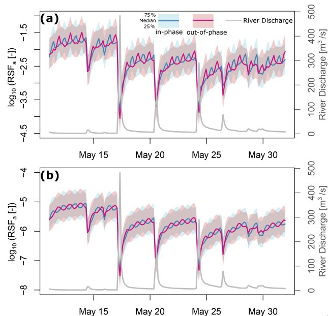
Figure 8. Reaction significance factors per unit area ( \text{RSF}_a ) for denitrification potentials from 15 to 30 May 2017. (a) \text{RSF}_a under gaining conditions. (b) \text{RSF}_a under losing conditions. The results are selected arbitrarily with the considerations of figure clarity
