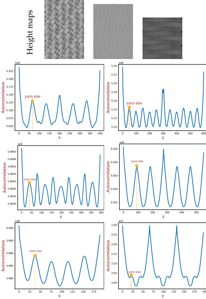
Fig. 4: Automatic selection of the size of our height-map-smoothing kernel: we select filter size automatically for fabrics with strong patterns by analyzing the height map’s horizontal and vertical autocorrelations via Eq. 4. In this example, each row of plots corresponds to a height map shown on the top.
