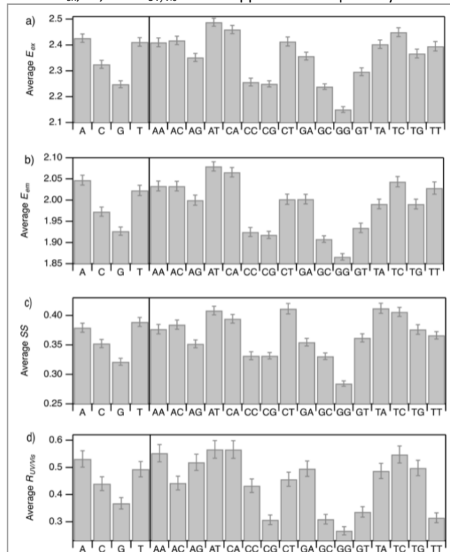
Figure 5: Mean values of (a) E_{ex} , (b) E_{em} , (c) SS , and (d) R_{UV/vis} for each instance of the four nucleobases and the 16 possible two-base motifs in the set of DNA template sequences for the 305 spectrally pure Ag N -DNAs. Error bars represent standard error, as a measure of precision of the mean.
