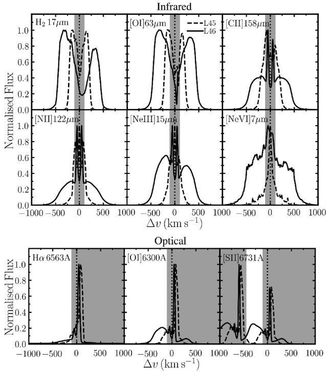
Figure 1. Continuum-subtracted spectra of six infrared emission lines (top two rows) and three optical emission lines (bottom row) commonly observed in AGN, from the simulations L45 (dashed curves) and L46 (solid curves), normalized to the maximum flux in each spectrum. These represent a subset of the lines that we study in this paper; the spectra from the full sample of 24 lines can be found in Appendix A. The vertical dotted line in each panel indicates the line centre. The broad component of these lines arises from the outflowing shell, with velocities extending up to \approx 300 and \approx 700 \text{km s}^{-1} in L45 and L46, respectively. However, central velocities at |\Delta v| \leq 100 \text{km s}^{-1} are typically dominated by narrow components from the ambient ISM. The grey shaded bands indicate velocity ranges that are excluded for the remainder of our analysis, to focus on the outflow component.
