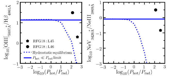
Figure 11. The line ratios [\text{O III}]_{5007\text{\AA}} / \text{H}\beta_{4861\text{\AA}} (left) and \text{Ne V}_{3426\text{\AA}} / \text{Ne III}_{3869\text{\AA}} (right) plotted against the ratio of hot gas pressure to radiation pressure ( P_{\text{hot}}/P_{\text{rad}} ). The black symbols show our simulations, while the blue dotted curves show the line ratios in an idealized CLOUDY photoionization model in hydrostatic equilibrium based on Stern et al. (2016) using the Sazonov et al. (2004) average quasar spectrum. The line ratios in the P_{\text{hot}} \ll P_{\text{rad}} (i.e. RPC) limit of the CLOUDY model are indicated by the horizontal blue lines. The line ratios from the simulations bracket the RPC limit of the CLOUDY model, which means that we cannot use these particular ratios to distinguish between the hot gas pressure dominated limit and RPC.
