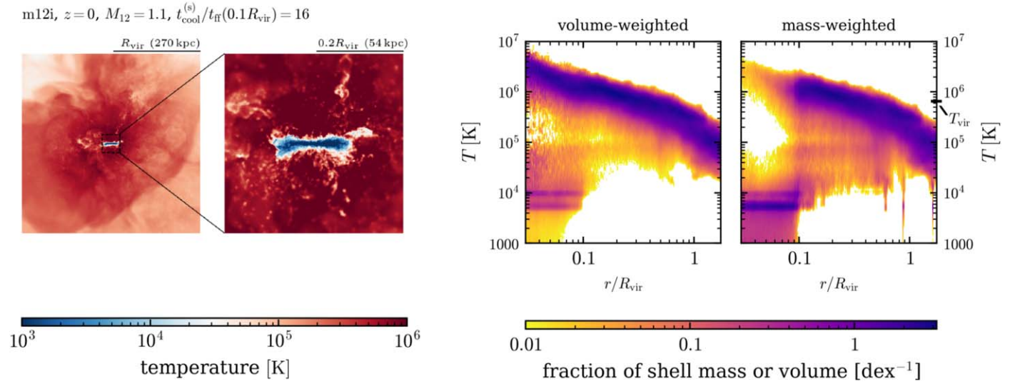
Figure 4. Temperature distribution in the main halo of m12i at z=0 , at which t_{\text{cool}}^{(s)}/t_{\text{ff}} = 16 at 0.1R_{\text{vir}} . Left panels: temperature map of a slice through the snapshot, oriented edge-on to the galaxy disk. The first panel spans the entire halo, and the second panel zooms in on the inner \pm 0.2R_{\text{vir}} . Right panels: temperature histograms of gas in shells at different radii, weighted by volume (third panel from the left) and weighted by mass (rightmost panel). Note that the hot phase temperature decreases from T \gtrsim 10^6 K at galaxy radii to T \approx 10^{5.5} K at \approx R_{\text{vir}} and dominates by volume on both halo and galaxy scales and by mass in the halo. The cool phase forms a prominent disk on galaxy scales and is entirely negligible by volume in the halo.
