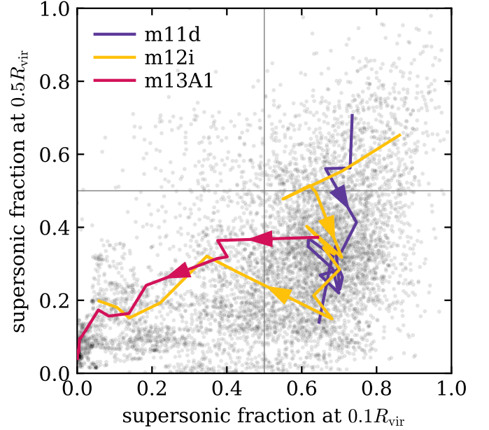
Figure 12. Volume fraction of supersonic gas in the inner and outer halo. Gray markers denote snapshots from all 16 simulations. Colored lines and arrows show the tracks of three individual simulations using the median values in windows of 1 Gyr (m11d and m12i) and windows of 500 Myr (m13A1). The tendency of the tracks to go through the lower right quadrant of the plot, rather than through the upper left quadrant, indicates that the quasi-static virialized CGM forms from the outside in rather than from the inside out.
