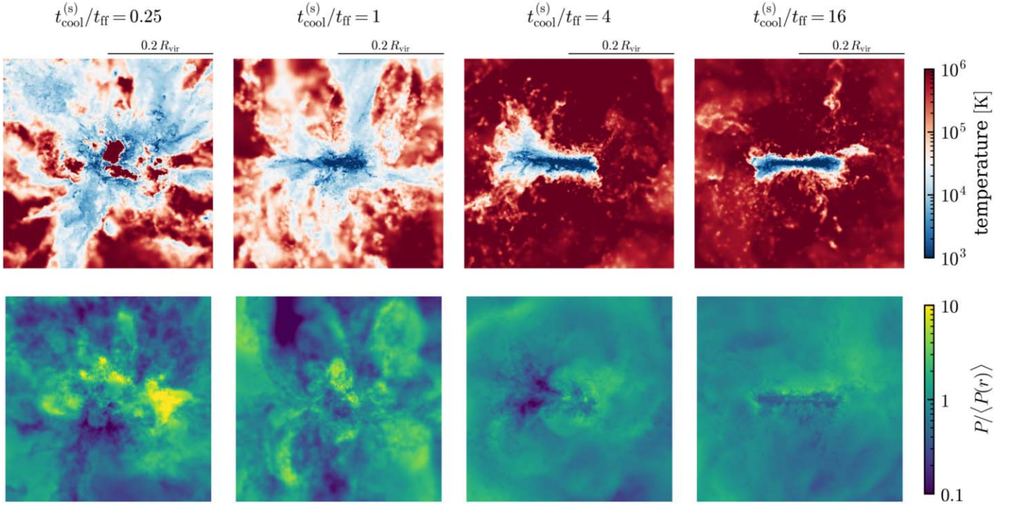
Figure 8. Temperature (top) and pressure fluctuations (bottom) in the inner halo vs. the ratio of cooling time to free-fall time. The panels show snapshots of the m12i simulation at z = 1, 0.4, 0.1 , and 0 from left to right. The corresponding t_{\text{cool}}^{(s)}/t_{\text{ff}} at 0.1R_{\text{vir}} are noted on top. In the bottom row the pressure at each pixel is normalized by the average pressure at the same radius (Equation (21)). The images are oriented such that the angular momentum vector of galaxy gas is directed upward. Note that when t_{\text{cool}}^{(s)} exceeds t_{\text{ff}} the inner halo volume becomes uniformly hot, pressure fluctuations decrease, and a prominent disk appears.
