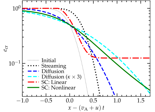
Figure B1. Illustration of the behaviour of the solutions for CR transport with \kappa_{\parallel} and v_{\text{st}} given by SC models (see Appendix B3). We evolve a one-dimensional toy model with parallel fields ( \hat{\mathbf{b}} = \hat{\mathbf{x}} = \hat{\nabla}_{\parallel} e_{\text{cr}} ) and constant v_A , u , and other background properties. Taking \tilde{c} \rightarrow \infty in equation (2), so \mathbf{F} = F \hat{\mathbf{x}} has its local-equilibrium value, and neglecting sources and sinks, the CR transport equations reduce to (\partial_t + [v_A + u] \partial_x) e_{\text{cr}} = -\partial_x F . We consider an initial step-function-like e_{\text{cr}} = 0.5 \text{ erfc}(x/0.3) evolved to time t = 0.5 (arbitrary units) assuming (1) traditional streaming/advection with F = v_{\text{adv}} e_{\text{cr}} where v_{\text{adv}} = 1 is a constant; (2) traditional diffusion with F = -\kappa \partial_x e_{\text{cr}} and \kappa = 1 or =3 is constant; (3) the expression for F = F_{\Gamma} = \kappa_{\parallel} \partial_x e_{\text{cr}} = (4 c r_L e_B / \pi v_A) \Gamma_{\text{eff}} actually given by SC models (equation B5) assuming linear-damping terms dominate so \Gamma_{\text{eff}} = \Gamma_{\text{in}} + \Gamma_{\text{turb}} + \Gamma_{\text{LL}} , giving \partial_x F = -C_L \text{SIGN}(\partial_x e_{\text{cr}}) with C_L = 1/2 ; (4) the expression for SC (equation B5) with non-linear terms dominant ( \Gamma_{\text{eff}} = \Gamma_{\text{NLL}} ), so F_{\Gamma} = C_{\text{NL}} |\partial_x e_{\text{cr}}|^{1/2} with C_{\text{NL}} = 1 . These are the simplest expressions that produce non-trivial behaviour for each version of the equations, and we choose v_{\text{adv}} , \kappa , C_L , C_{\text{NL}} so that the ‘effective’ transport speed \bar{v}_{\text{st, eff}} is the same around (x, t) = (0, 0) . Despite the fact that we can write the SC scalings as a ‘diffusive’ \kappa_{\parallel} (equation 7) or ‘super-Alfvénic streaming’ \bar{v}_{\text{st}} (equation 9), the behaviour of even the simplest solutions is not the same as true diffusion or streaming/advection equations.
